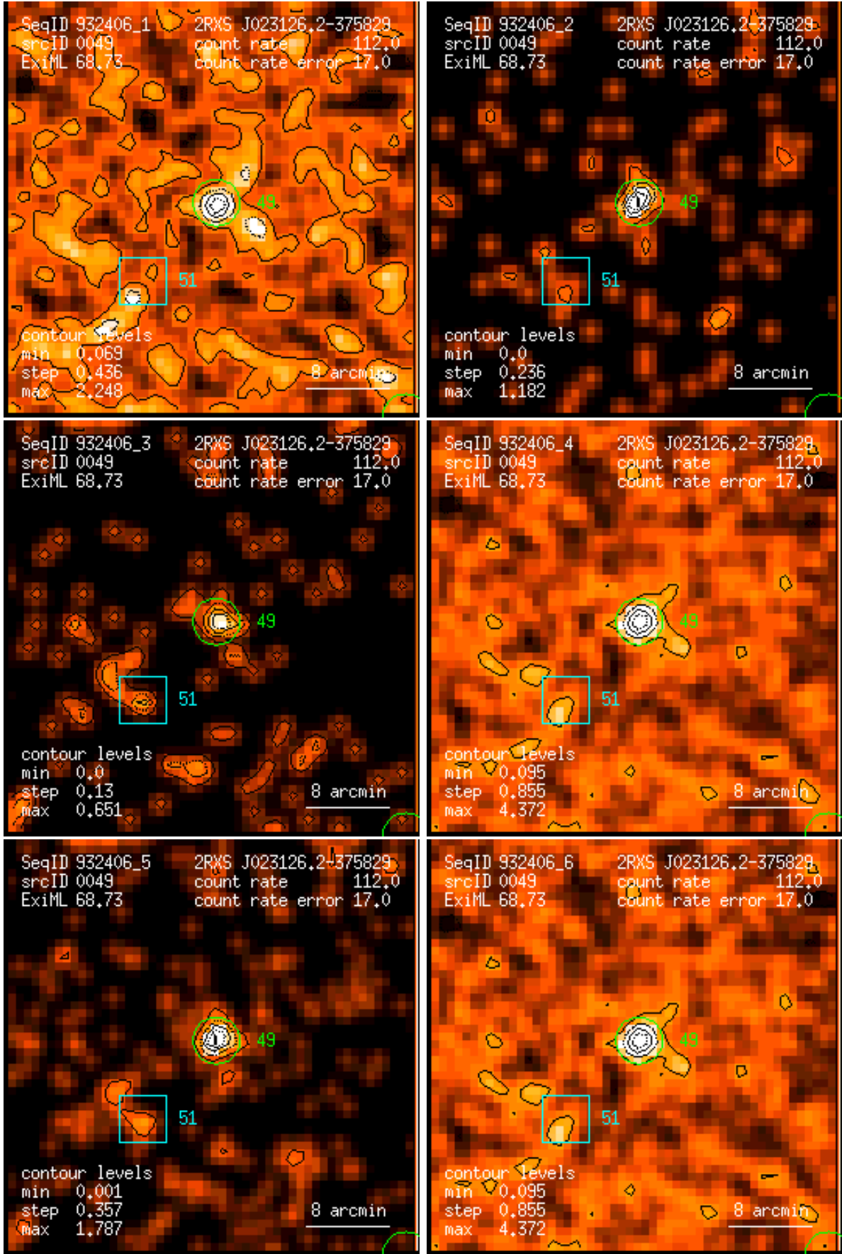
Figure 49: RASS 932406: detection 0049: band rate images, Gaussian filter: (1) PSPC channels 11 – 41, (2) 52 – 90, (3) 91 – 201, (4) 11 – 235, (5) 52 – 201, (6) 11 – 201. Broad band rates in counts/ks. Band rate contour levels in counts/ks/arcmin 2 .
