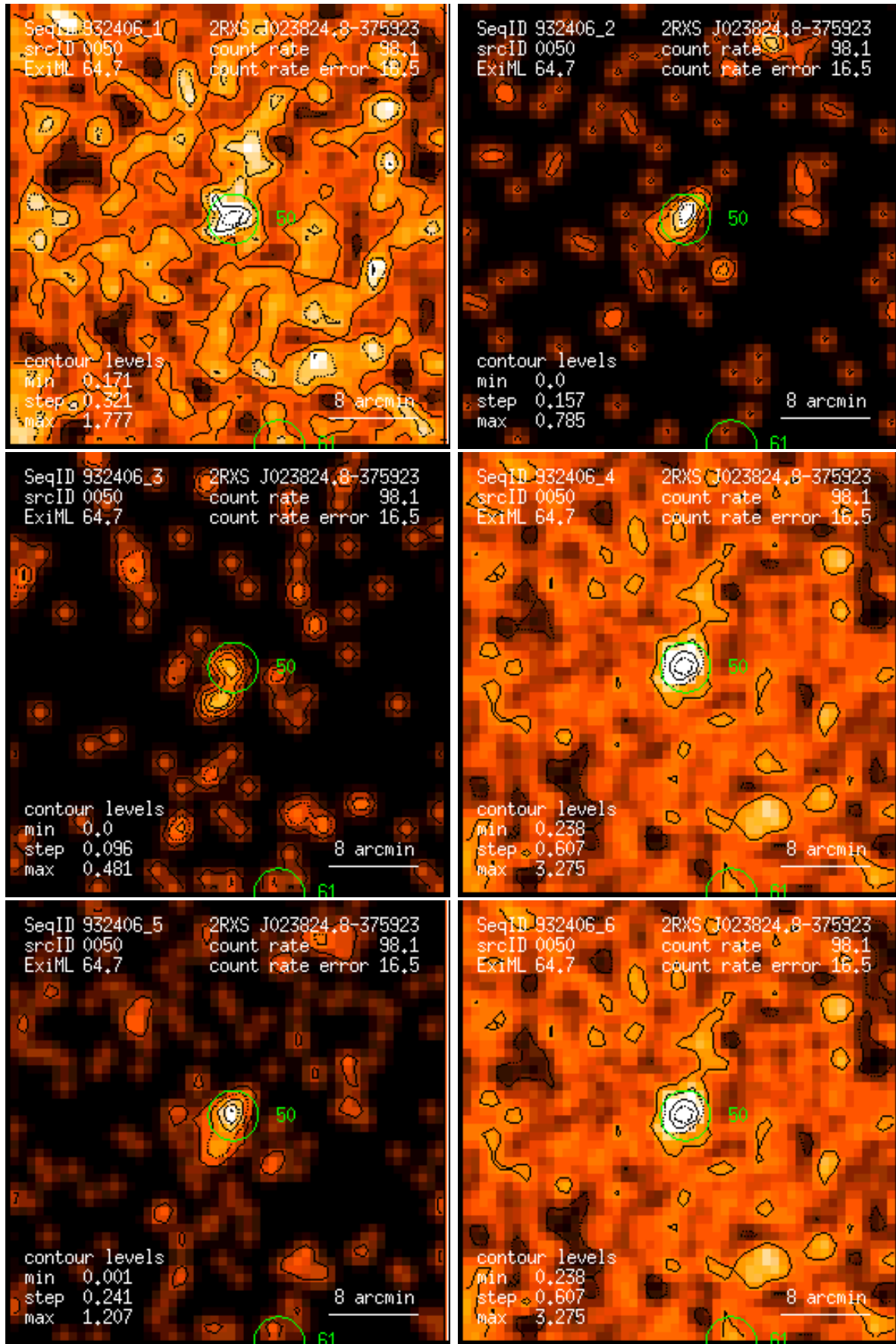
Figure 50: RASS 932406: detection 0050: band rate images, Gaussian filter: (1) PSPC channels 11 – 41, (2) 52 – 90, (3) 91 – 201, (4) 11 – 235, (5) 52 – 201, (6) 11 – 201. Broad band rates in counts/ks. Band rate contour levels in counts/ks/arcmin 2 .
