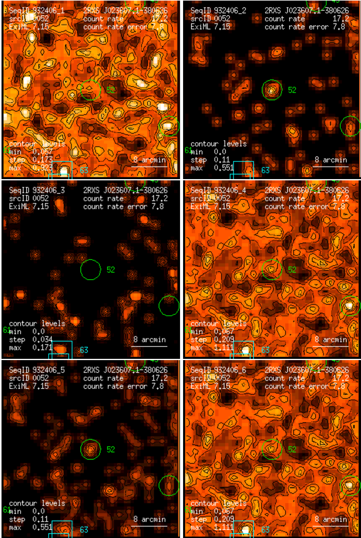
Figure 52: RASS 932406: detection 0052: band rate images, Gaussian filter: (1) PSPC channels 11 – 41, (2) 52 – 90, (3) 91 – 201, (4) 11 – 235, (5) 52 – 201, (6) 11 – 201. Broad band rates in counts/ks. Band rate contour levels in counts/ks/arcmin 2 .
