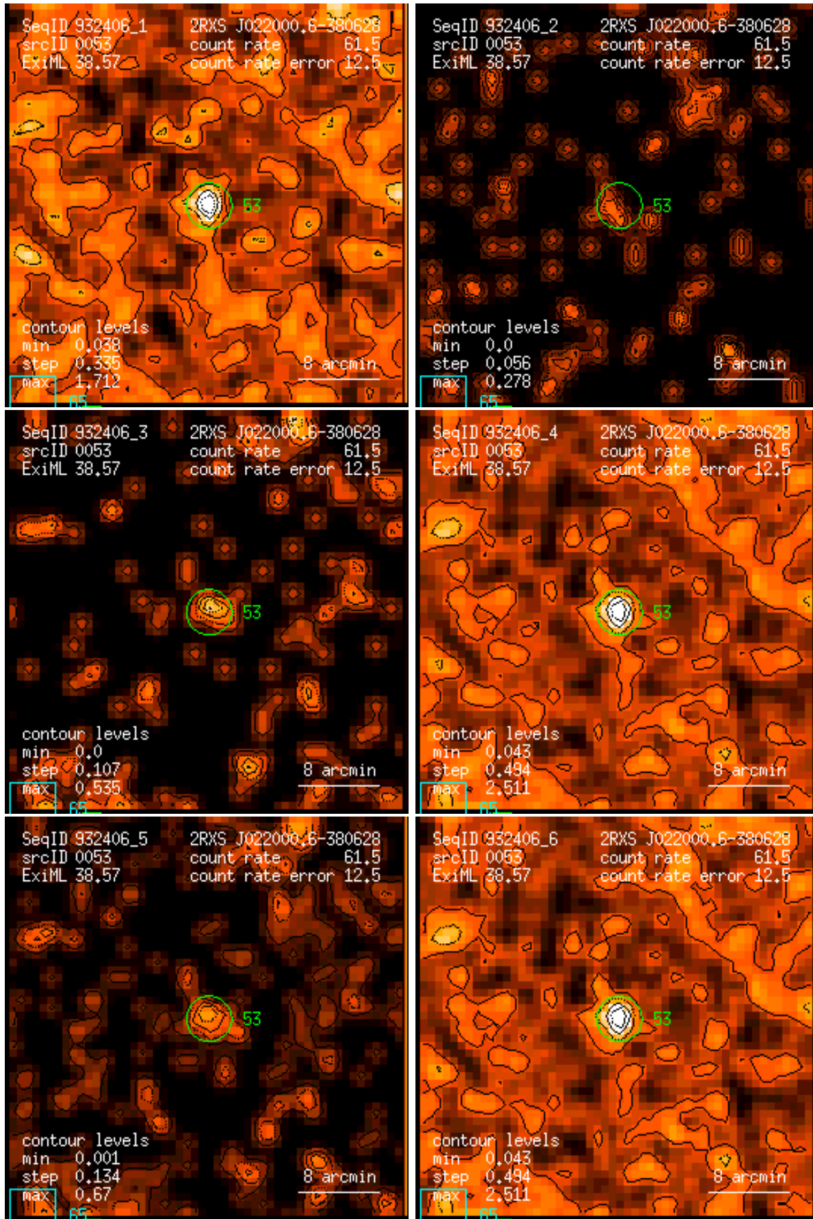
Figure 53: RASS 932406: detection 0053: band rate images, Gaussian filter: (1) PSPC channels 11 – 41, (2) 52 – 90, (3) 91 – 201, (4) 11 – 235, (5) 52 – 201, (6) 11 – 201. Broad band rates in counts/ks. Band rate contour levels in counts/ks/arcmin 2 .
