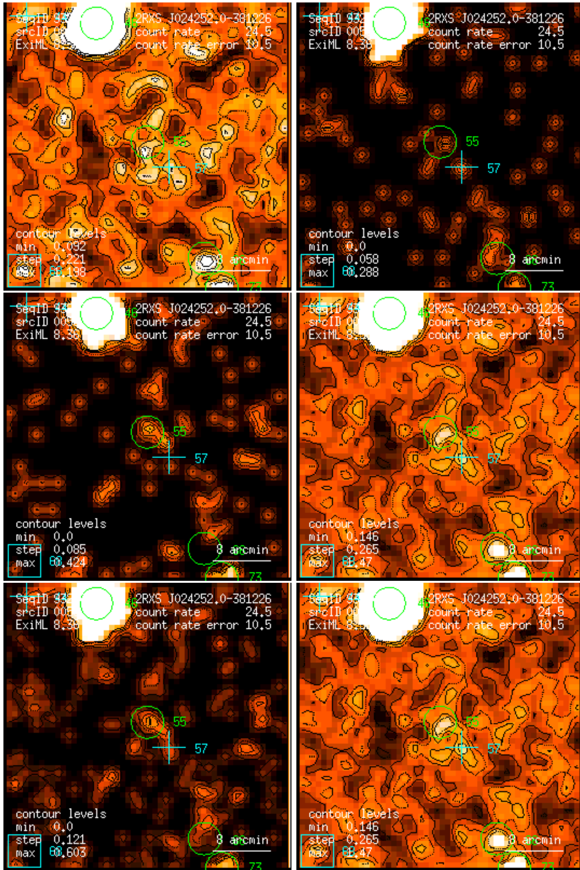
Figure 55: RASS 932406: detection 0055: band rate images, Gaussian filter: (1) PSPC channels 11 – 41, (2) 52 – 90, (3) 91 – 201, (4) 11 – 235, (5) 52 – 201, (6) 11 – 201. Broad band rates in counts/ks. Band rate contour levels in counts/ks/arcmin 2 .
