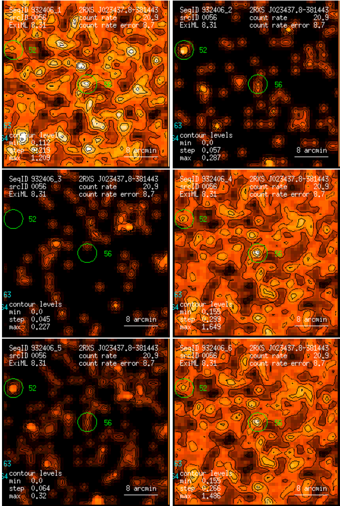
Figure 56: RASS 932406: detection 0056: band rate images, Gaussian filter: (1) PSPC channels 11 – 41, (2) 52 – 90, (3) 91 – 201, (4) 11 – 235, (5) 52 – 201, (6) 11 – 201. Broad band rates in counts/ks. Band rate contour levels in counts/ks/arcmin 2 .
