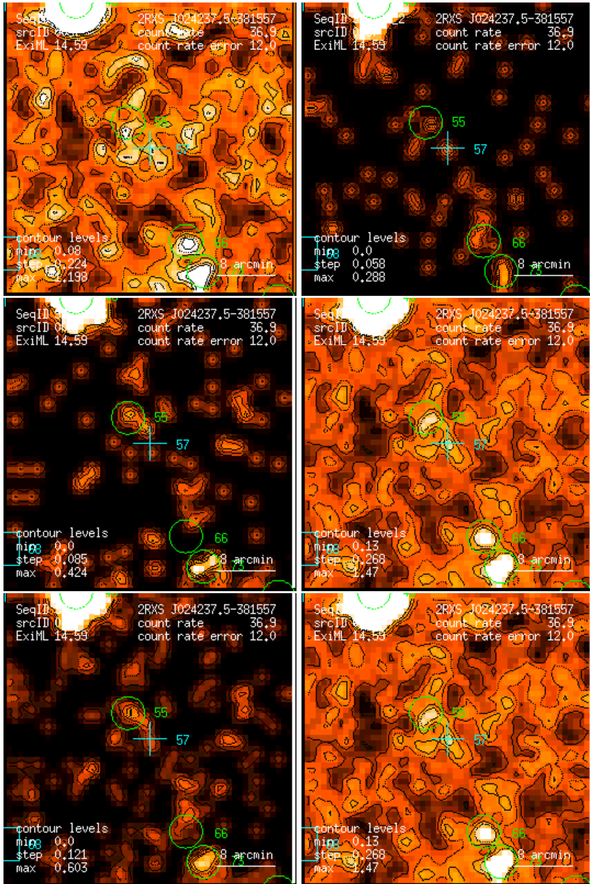
Figure 57: RASS 932406: detection 0057: band rate images, Gaussian filter: (1) PSPC channels 11 – 41, (2) 52 – 90, (3) 91 – 201, (4) 11 – 235, (5) 52 – 201, (6) 11 – 201. Broad band rates in counts/ks. Band rate contour levels in counts/ks/arcmin 2 .
