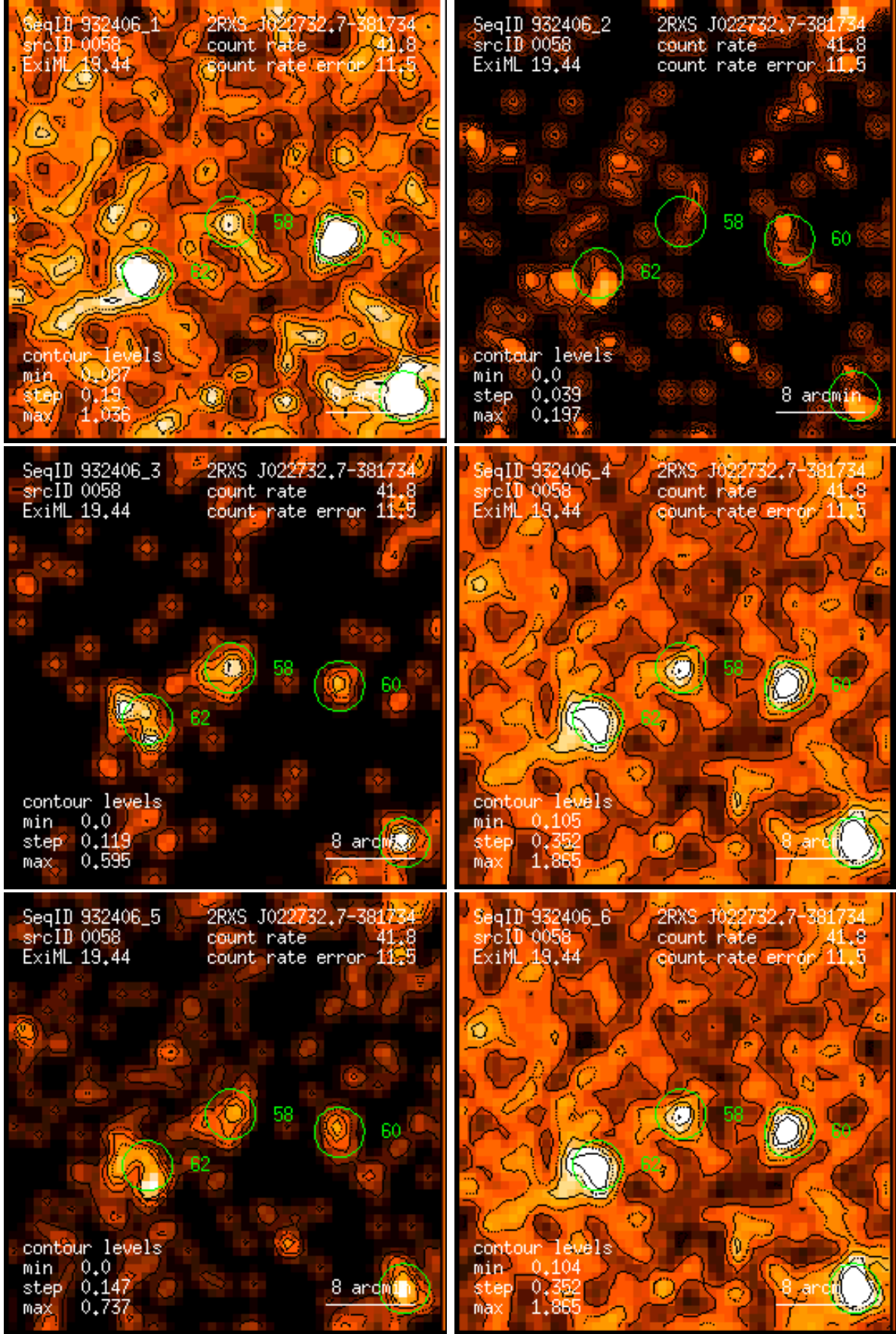
Figure 58: RASS 932406: detection 0058: band rate images, Gaussian filter: (1) PSPC channels 11 – 41, (2) 52 – 90, (3) 91 – 201, (4) 11 – 235, (5) 52 – 201, (6) 11 – 201. Broad band rates in counts/ks. Band rate contour levels in counts/ks/arcmin 2 .
