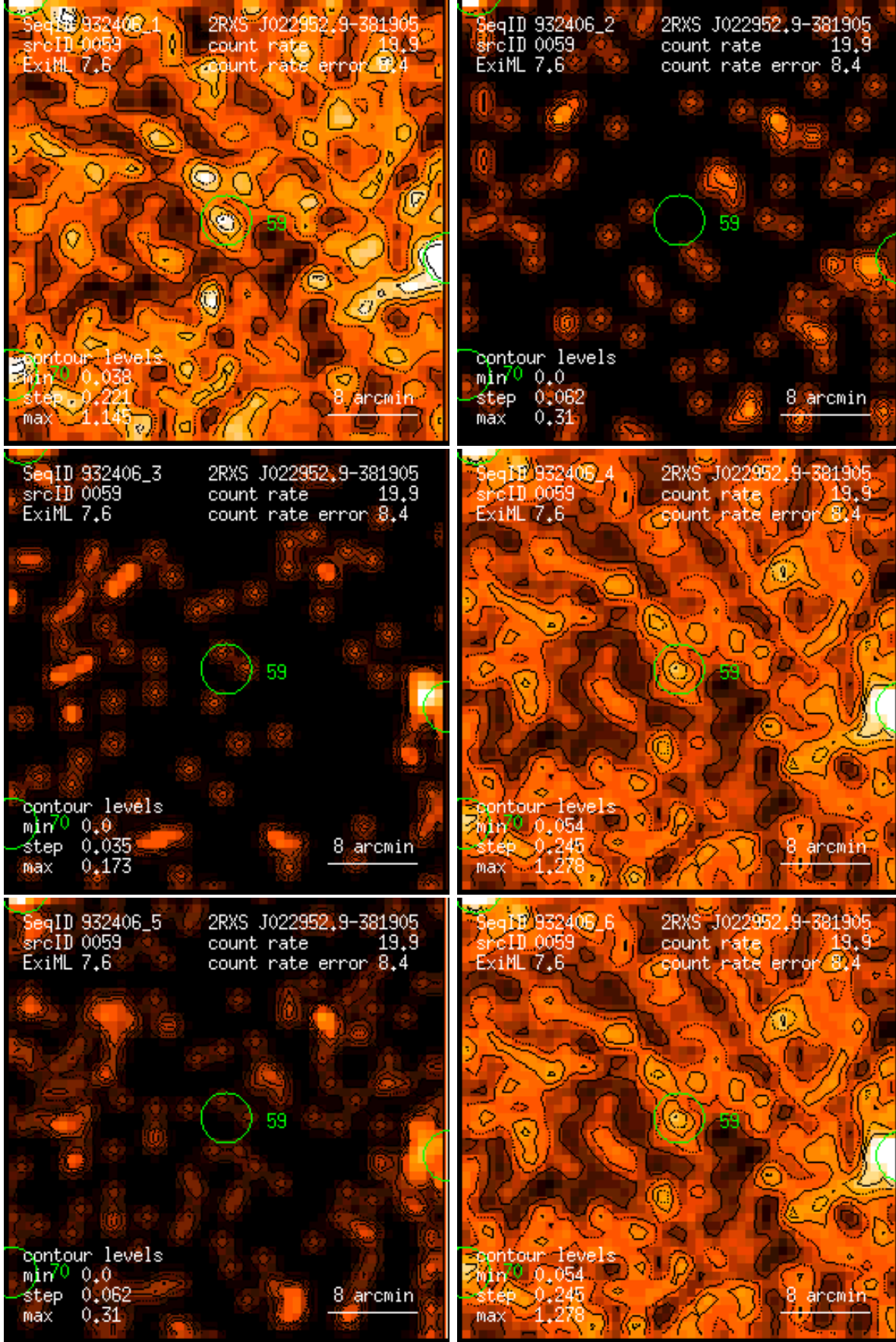
Figure 59: RASS 932406: detection 0059: band rate images, Gaussian filter: (1) PSPC channels 11 – 41, (2) 52 – 90, (3) 91 – 201, (4) 11 – 235, (5) 52 – 201, (6) 11 – 201. Broad band rates in counts/ks. Band rate contour levels in counts/ks/arcmin 2 .
