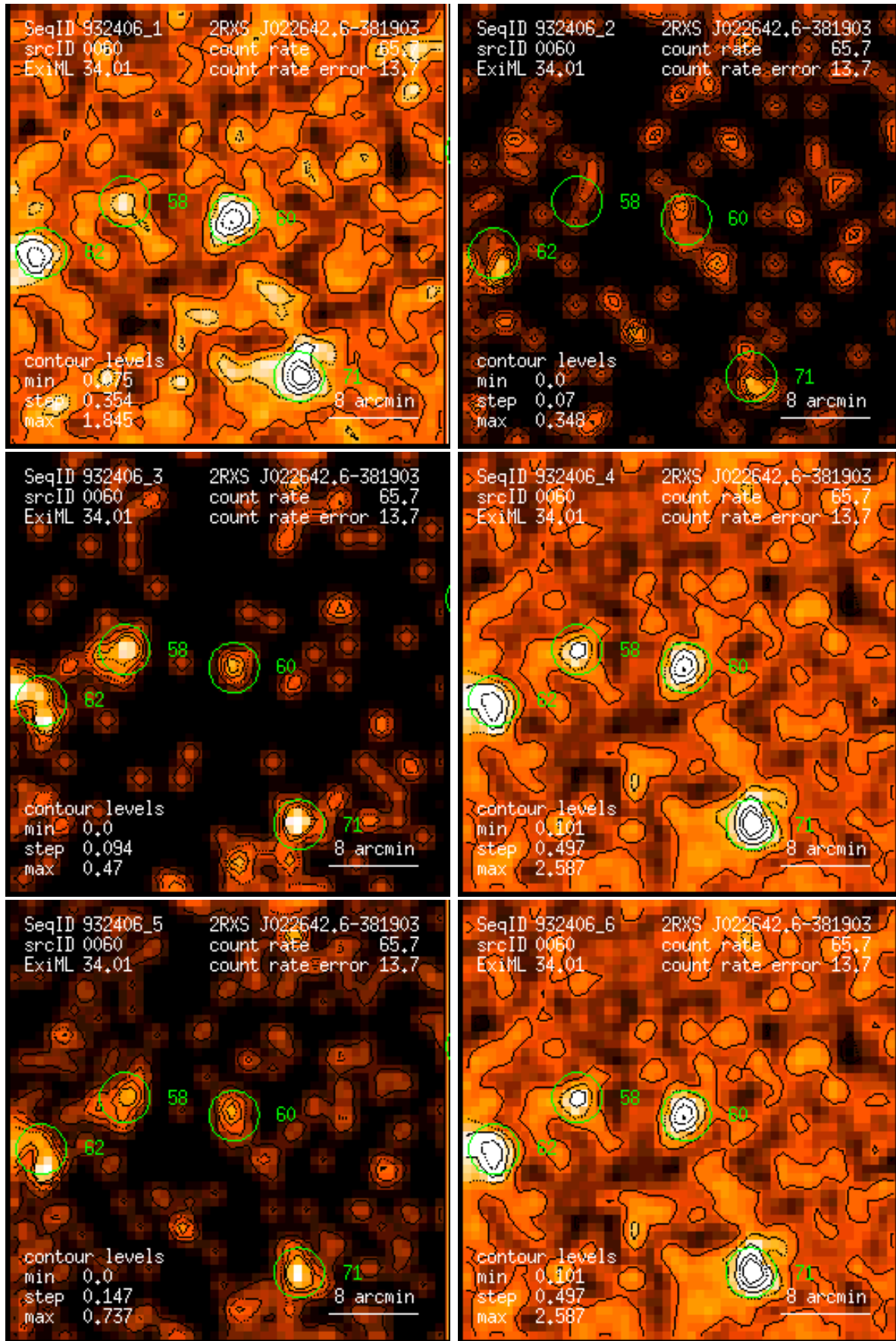
Figure 60: RASS 932406: detection 0060: band rate images, Gaussian filter: (1) PSPC channels 11 – 41, (2) 52 – 90, (3) 91 – 201, (4) 11 – 235, (5) 52 – 201, (6) 11 – 201. Broad band rates in counts/ks. Band rate contour levels in counts/ks/arcmin 2 .
