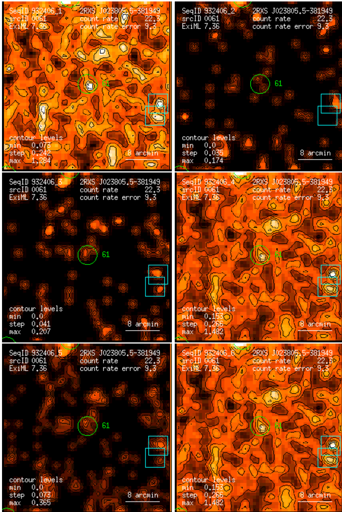
Figure 61: RASS 932406: detection 0061: band rate images, Gaussian filter: (1) PSPC channels 11 – 41, (2) 52 – 90, (3) 91 – 201, (4) 11 – 235, (5) 52 – 201, (6) 11 – 201. Broad band rates in counts/ks. Band rate contour levels in counts/ks/arcmin 2 .
