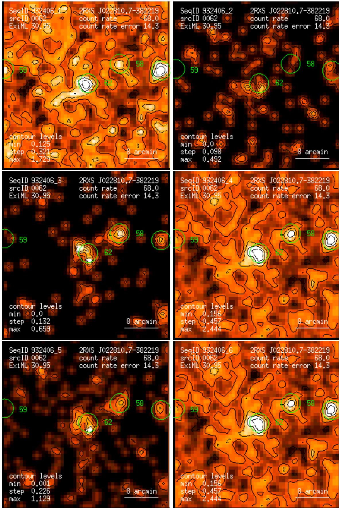
Figure 62: RASS 932406: detection 0062: band rate images, Gaussian filter: (1) PSPC channels 11 – 41, (2) 52 – 90, (3) 91 – 201, (4) 11 – 235, (5) 52 – 201, (6) 11 – 201. Broad band rates in counts/ks. Band rate contour levels in counts/ks/arcmin 2 .
