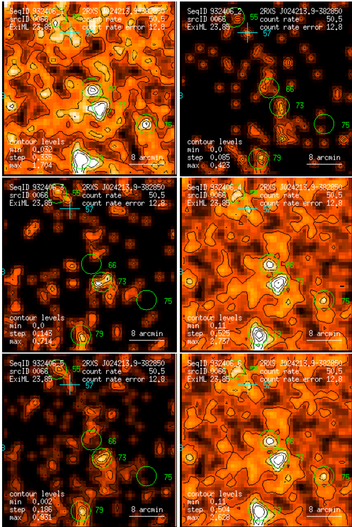
Figure 66: RASS 932406: detection 0066: band rate images, Gaussian filter: (1) PSPC channels 11 – 41, (2) 52 – 90, (3) 91 – 201, (4) 11 – 235, (5) 52 – 201, (6) 11 – 201. Broad band rates in counts/ks. Band rate contour levels in counts/ks/arcmin 2 .
