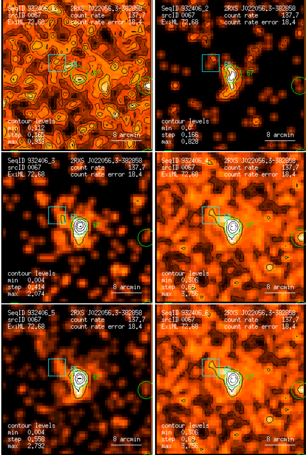
Figure 67: RASS 932406: detection 0067: band rate images, Gaussian filter: (1) PSPC channels 11 – 41, (2) 52 – 90, (3) 91 – 201, (4) 11 – 235, (5) 52 – 201, (6) 11 – 201. Broad band rates in counts/ks. Band rate contour levels in counts/ks/arcmin 2 .
