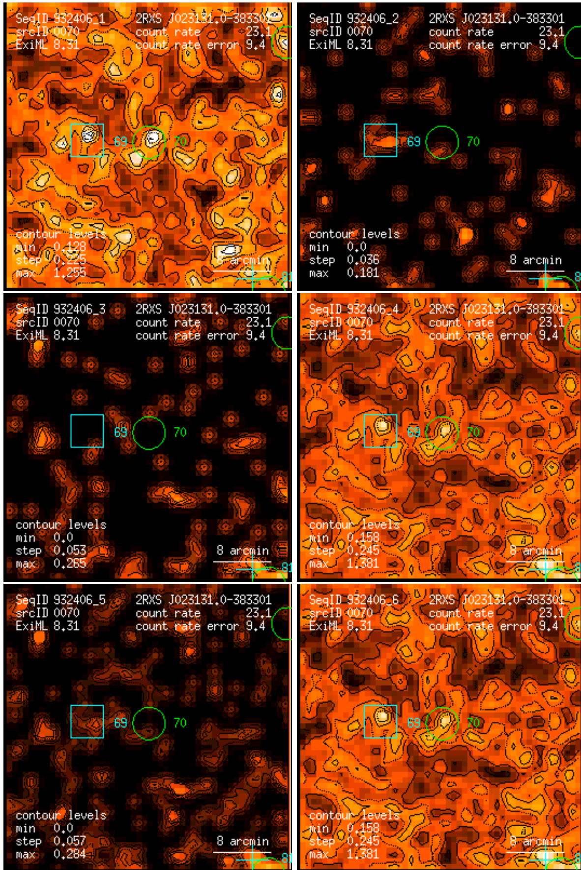
Figure 70: RASS 932406: detection 0070: band rate images, Gaussian filter: (1) PSPC channels 11 – 41, (2) 52 – 90, (3) 91 – 201, (4) 11 – 235, (5) 52 – 201, (6) 11 – 201. Broad band rates in counts/ks. Band rate contour levels in counts/ks/arcmin 2 .
