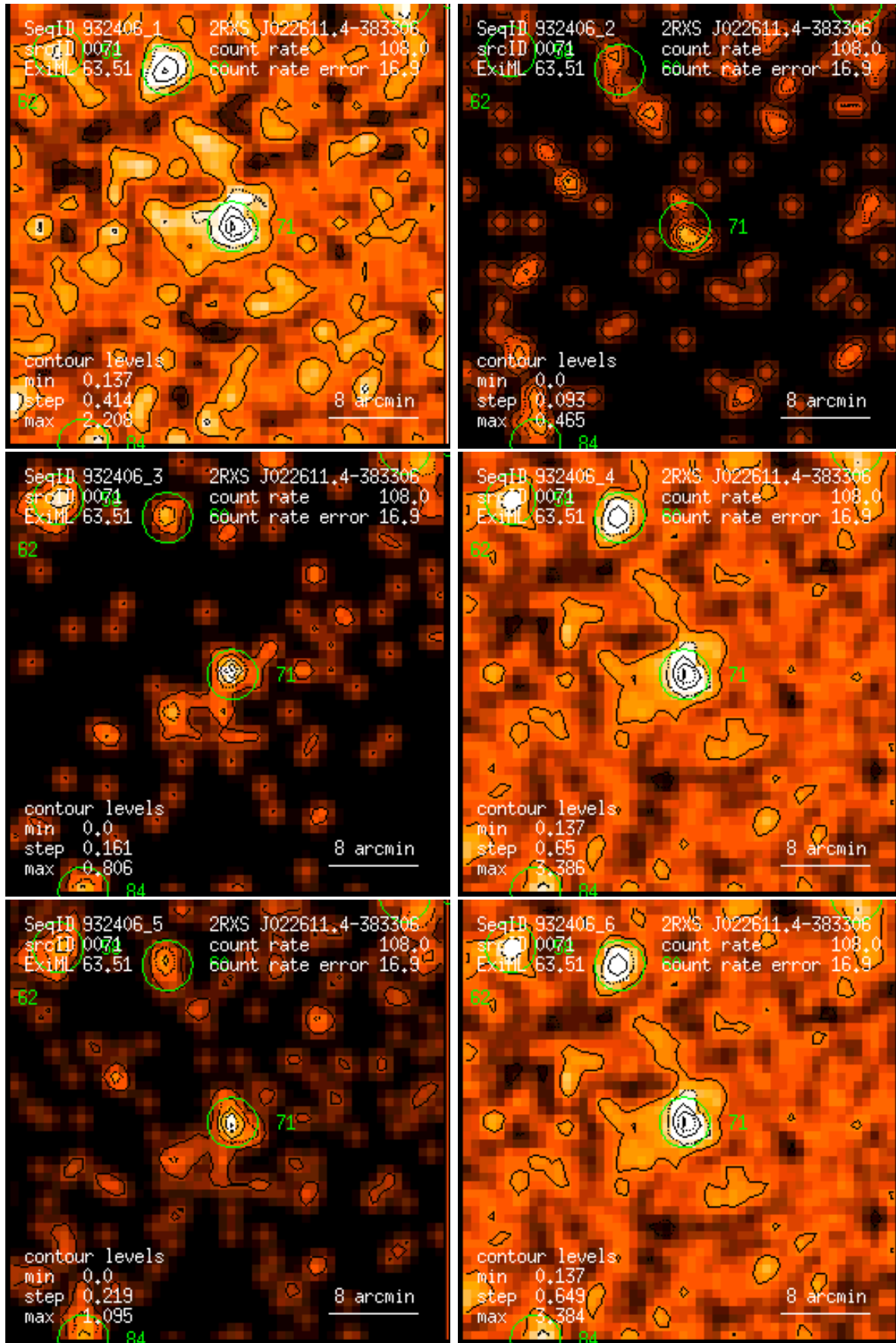
Figure 71: RASS 932406: detection 0071: band rate images, Gaussian filter: (1) PSPC channels 11 – 41, (2) 52 – 90, (3) 91 – 201, (4) 11 – 235, (5) 52 – 201, (6) 11 – 201. Broad band rates in counts/ks. Band rate contour levels in counts/ks/arcmin 2 .
