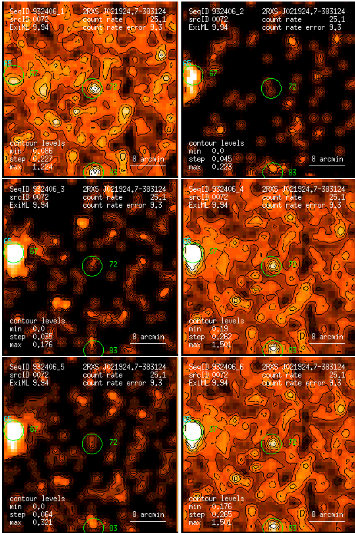
Figure 72: RASS 932406: detection 0072: band rate images, Gaussian filter: (1) PSPC channels 11 – 41, (2) 52 – 90, (3) 91 – 201, (4) 11 – 235, (5) 52 – 201, (6) 11 – 201. Broad band rates in counts/ks. Band rate contour levels in counts/ks/arcmin 2 .
