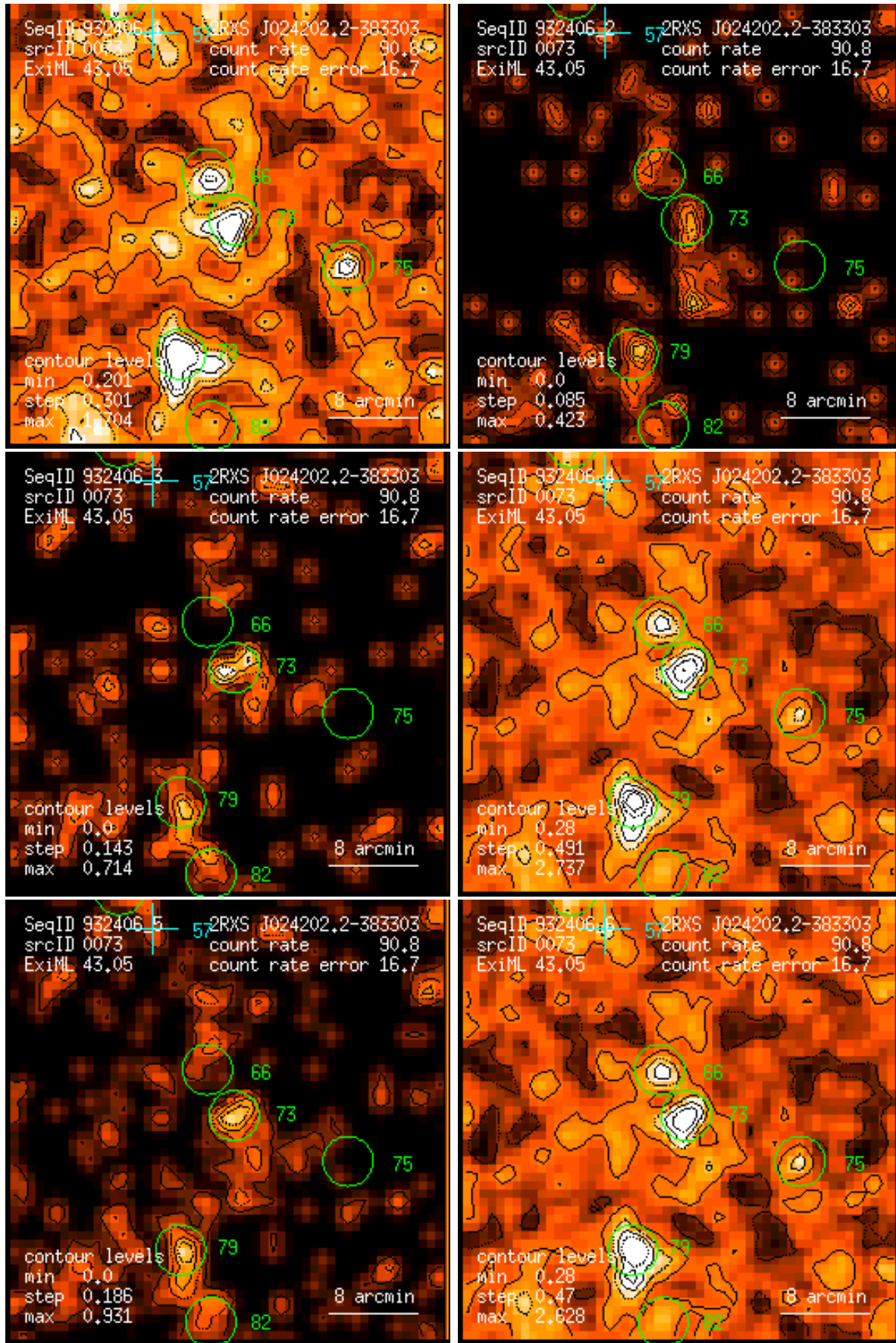
Figure 73: RASS 932406: detection 0073: band rate images, Gaussian filter: (1) PSPC channels 11 – 41, (2) 52 – 90, (3) 91 – 201, (4) 11 – 235, (5) 52 – 201, (6) 11 – 201. Broad band rates in counts/ks. Band rate contour levels in counts/ks/arcmin 2 .
