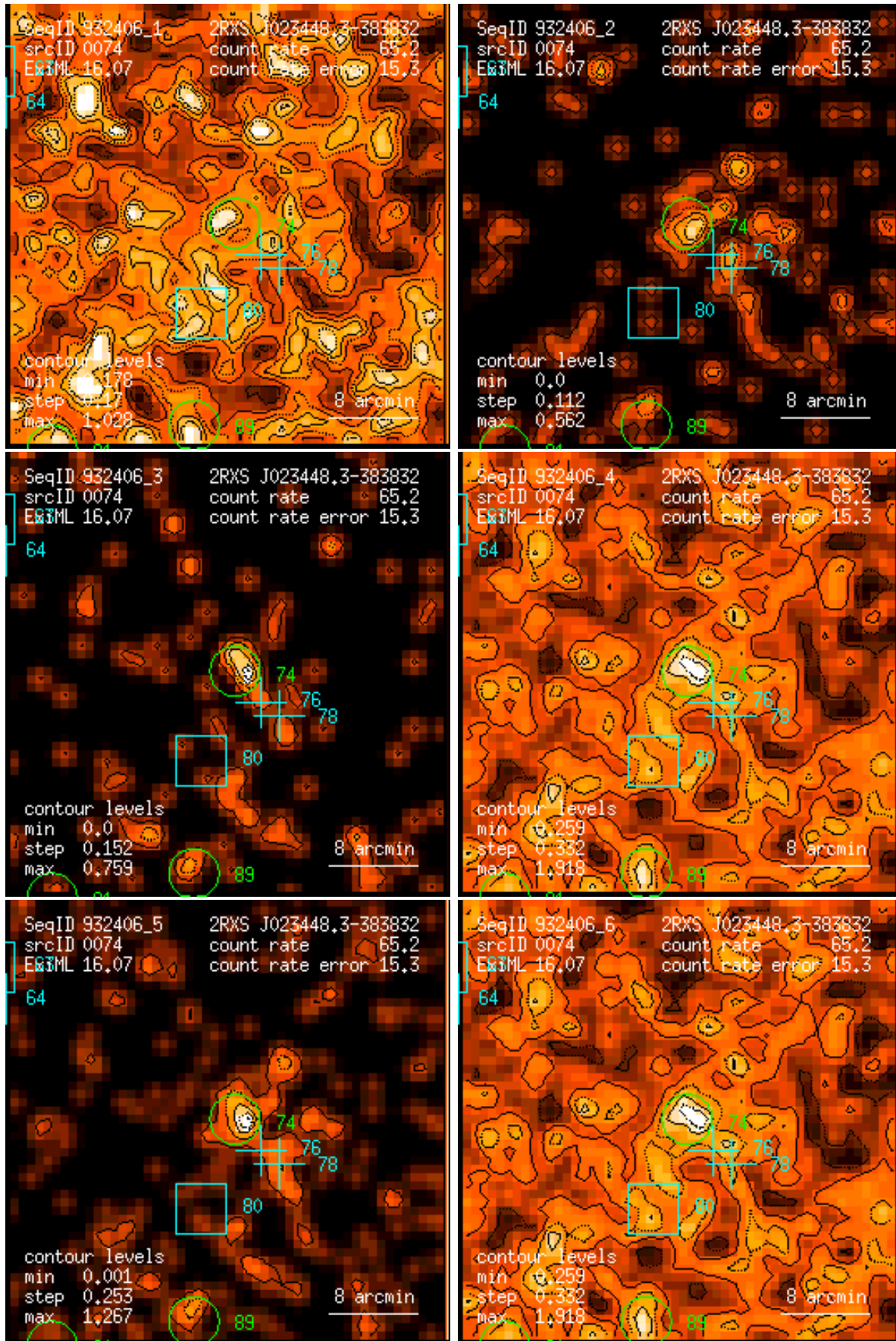
Figure 74: RASS 932406: detection 0074: band rate images, Gaussian filter: (1) PSPC channels 11 – 41, (2) 52 – 90, (3) 91 – 201, (4) 11 – 235, (5) 52 – 201, (6) 11 – 201. Broad band rates in counts/ks. Band rate contour levels in counts/ks/arcmin 2 .
