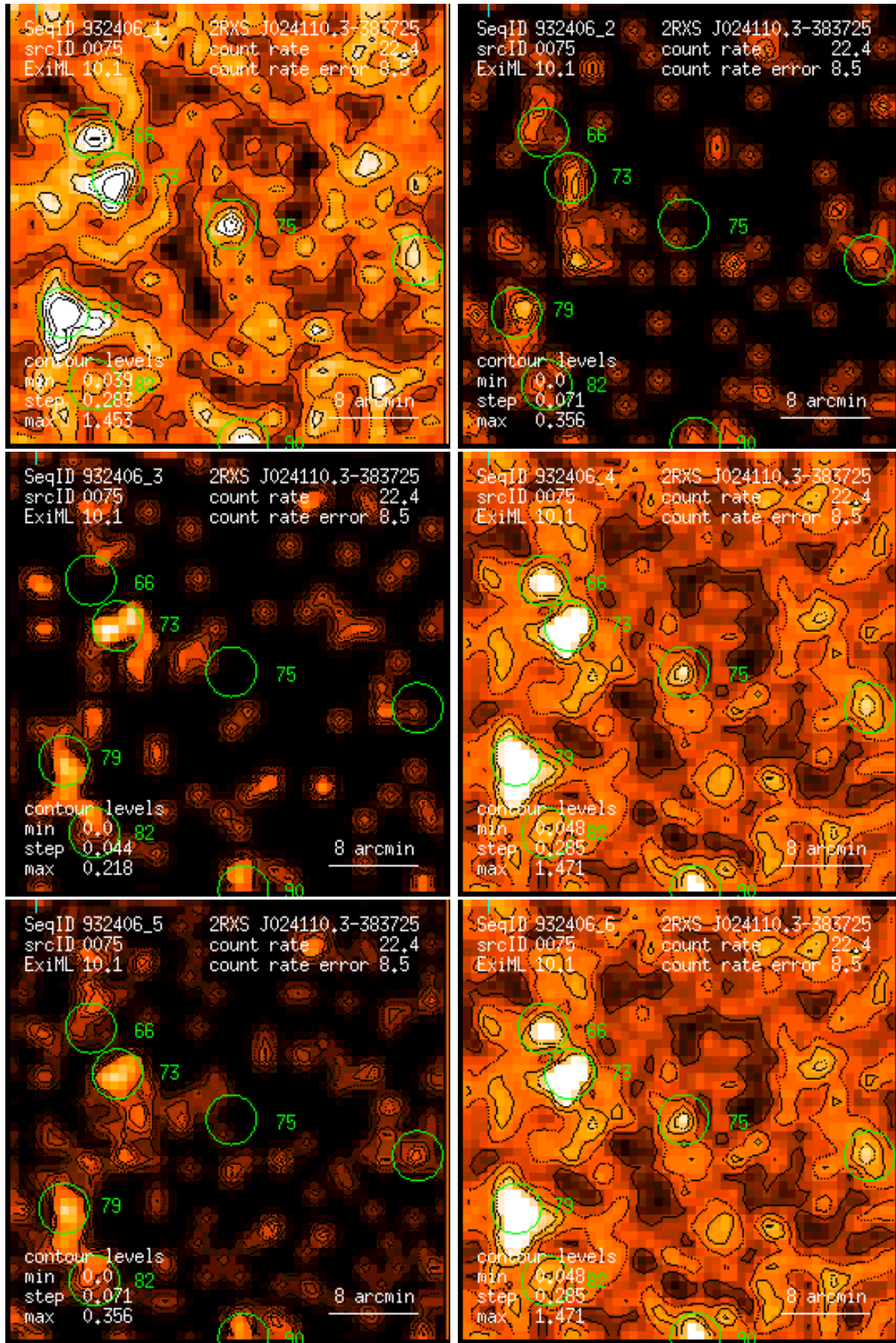
Figure 75: RASS 932406: detection 0075: band rate images, Gaussian filter: (1) PSPC channels 11 – 41, (2) 52 – 90, (3) 91 – 201, (4) 11 – 235, (5) 52 – 201, (6) 11 – 201. Broad band rates in counts/ks. Band rate contour levels in counts/ks/arcmin 2 .
