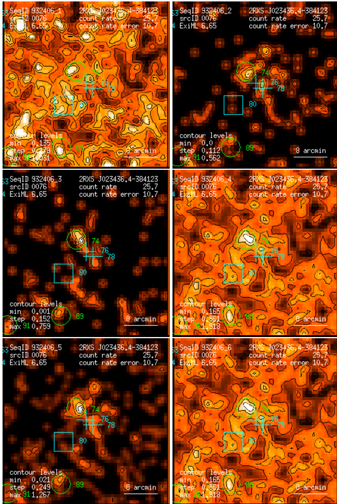
Figure 76: RASS 932406: detection 0076: band rate images, Gaussian filter: (1) PSPC channels 11 – 41, (2) 52 – 90, (3) 91 – 201, (4) 11 – 235, (5) 52 – 201, (6) 11 – 201. Broad band rates in counts/ks. Band rate contour levels in counts/ks/arcmin 2 .
