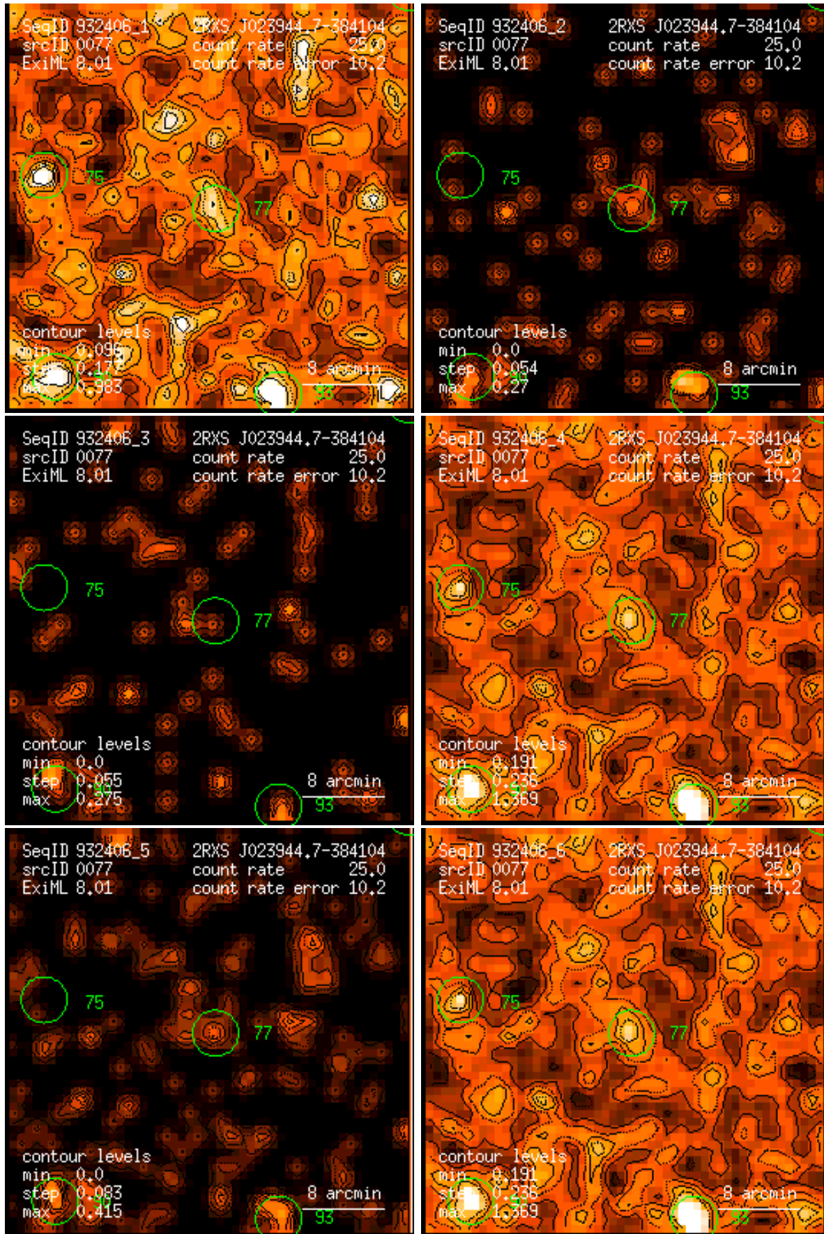
Figure 77: RASS 932406: detection 0077: band rate images, Gaussian filter: (1) PSPC channels 11 – 41, (2) 52 – 90, (3) 91 – 201, (4) 11 – 235, (5) 52 – 201, (6) 11 – 201. Broad band rates in counts/ks. Band rate contour levels in counts/ks/arcmin 2 .
