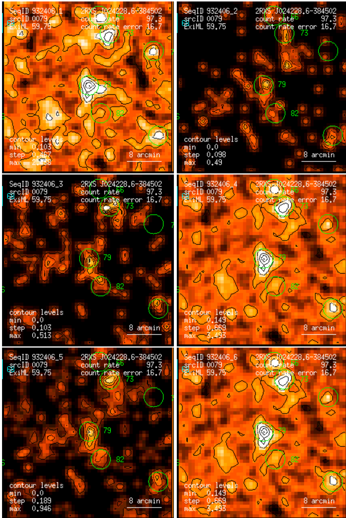
Figure 79: RASS 932406: detection 0079: band rate images, Gaussian filter: (1) PSPC channels 11 – 41, (2) 52 – 90, (3) 91 – 201, (4) 11 – 235, (5) 52 – 201, (6) 11 – 201. Broad band rates in counts/ks. Band rate contour levels in counts/ks/arcmin 2 .
