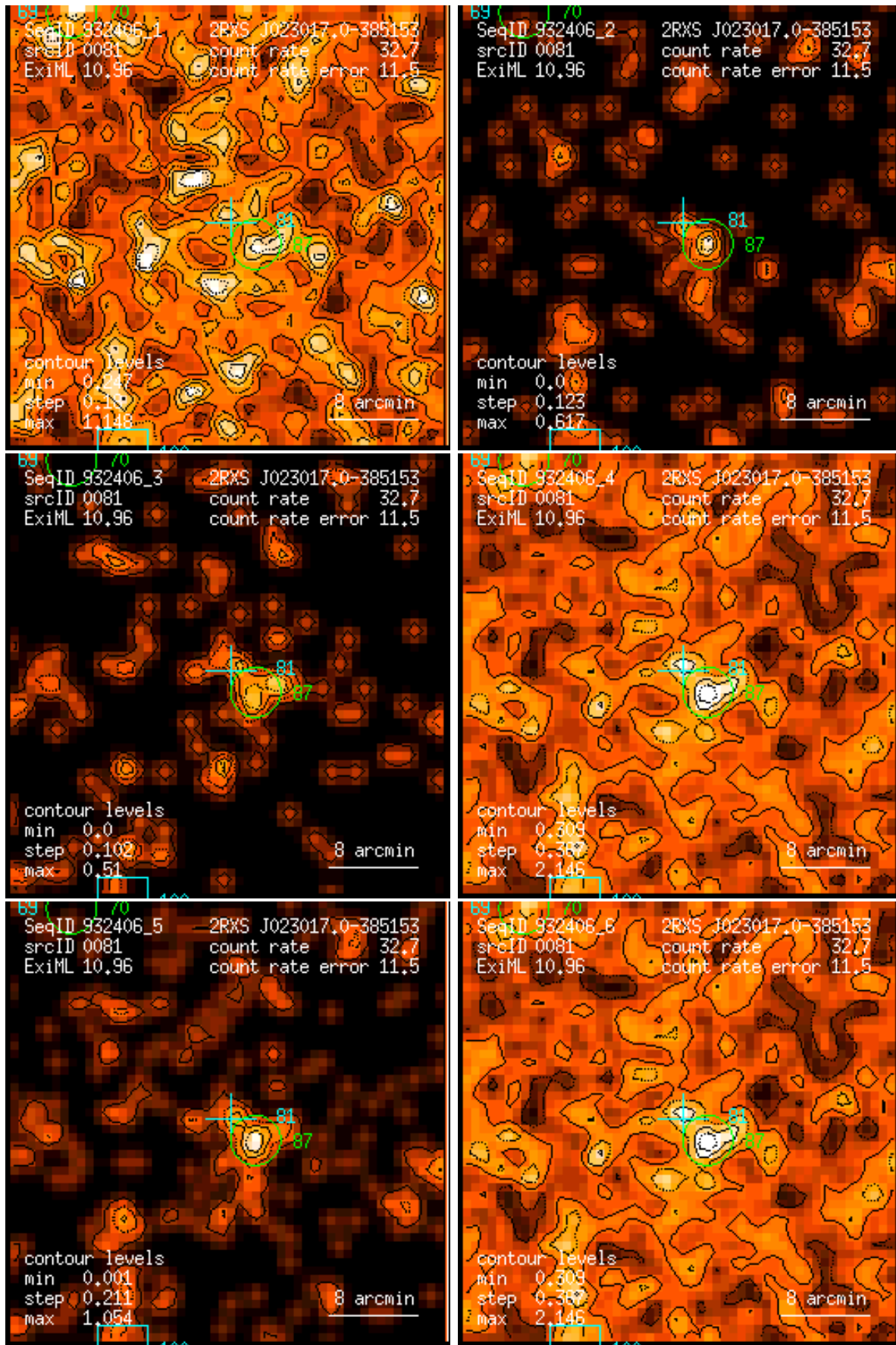
Figure 81: RASS 932406: detection 0081: band rate images, Gaussian filter: (1) PSPC channels 11 – 41, (2) 52 – 90, (3) 91 – 201, (4) 11 – 235, (5) 52 – 201, (6) 11 – 201. Broad band rates in counts/ks. Band rate contour levels in counts/ks/arcmin 2 .
