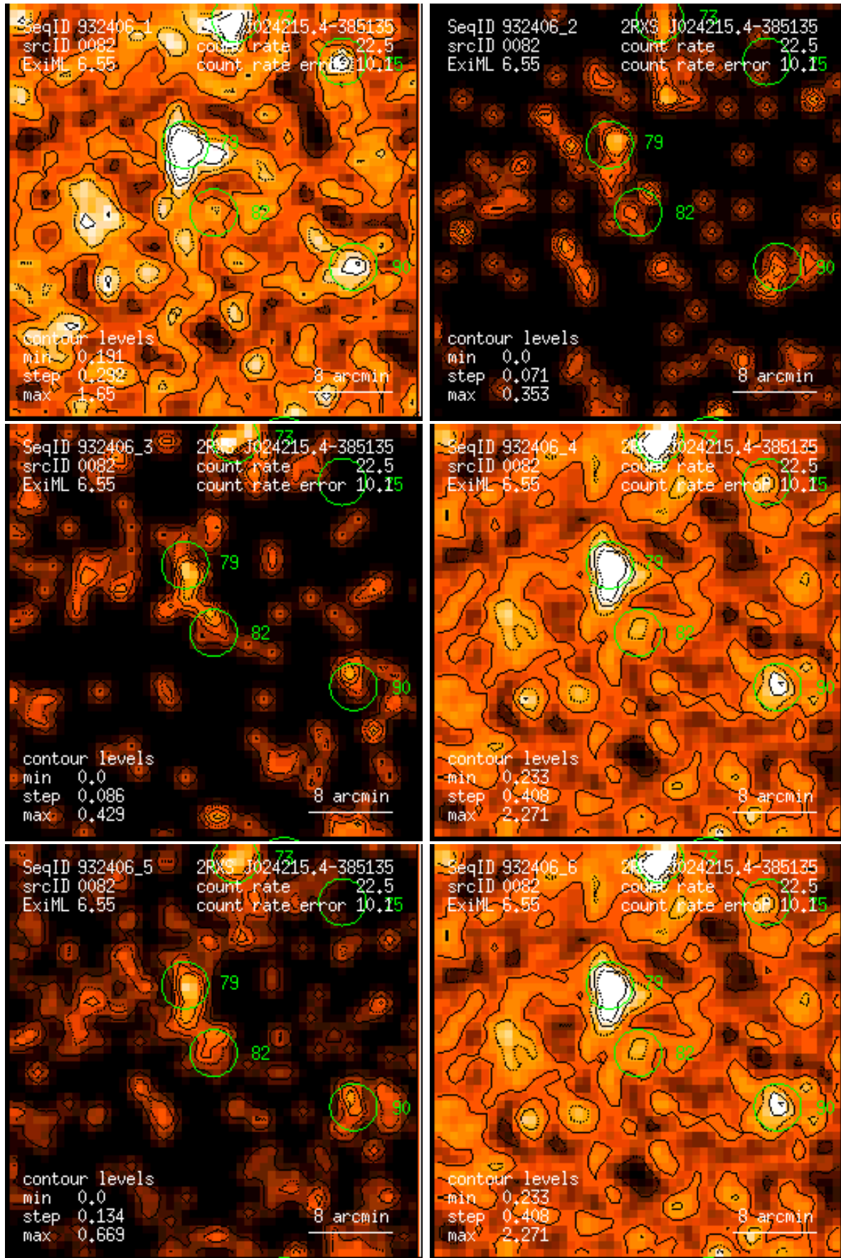
Figure 82: RASS 932406: detection 0082: band rate images, Gaussian filter: (1) PSPC channels 11 – 41, (2) 52 – 90, (3) 91 – 201, (4) 11 – 235, (5) 52 – 201, (6) 11 – 201. Broad band rates in counts/ks. Band rate contour levels in counts/ks/arcmin 2 .
