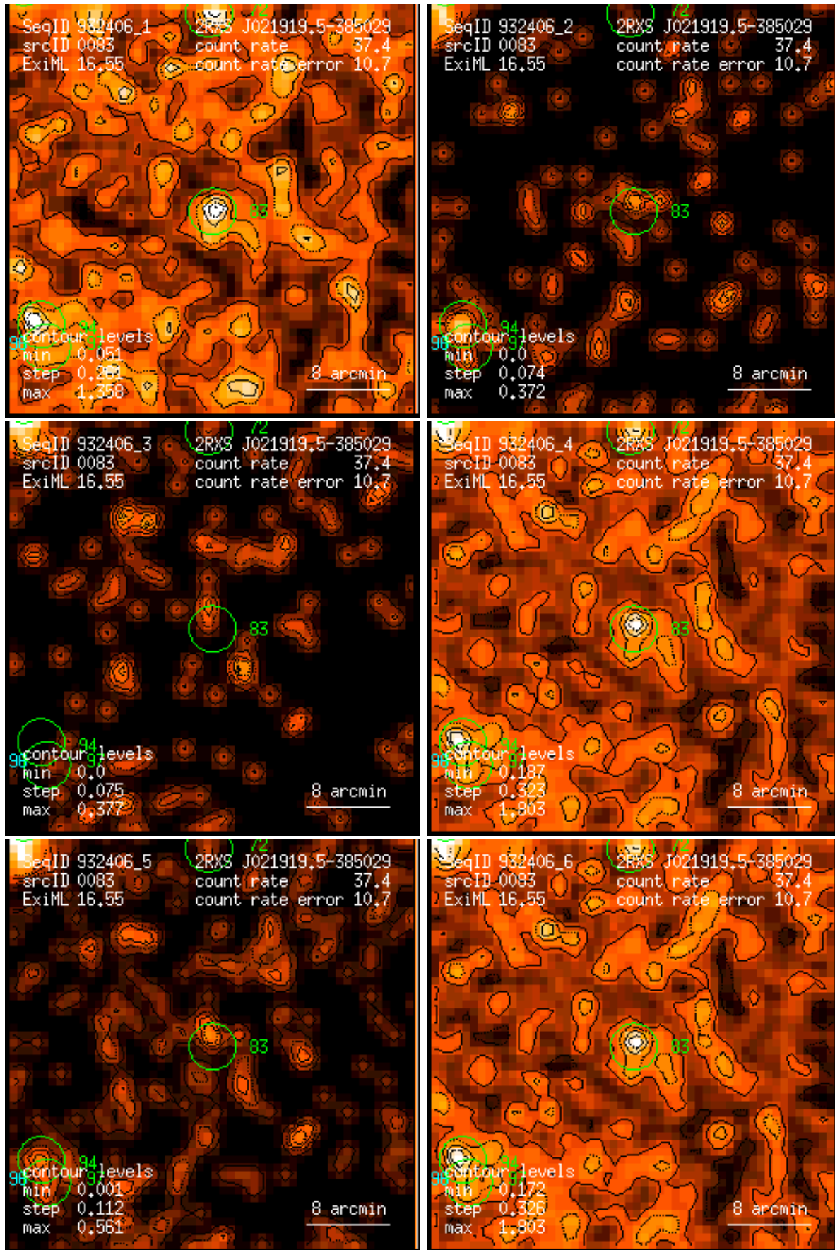
Figure 83: RASS 932406: detection 0083: band rate images, Gaussian filter: (1) PSPC channels 11 – 41, (2) 52 – 90, (3) 91 – 201, (4) 11 – 235, (5) 52 – 201, (6) 11 – 201. Broad band rates in counts/ks. Band rate contour levels in counts/ks/arcmin 2 .
