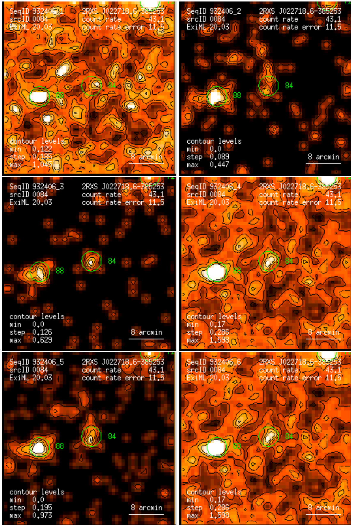
Figure 84: RASS 932406: detection 0084: band rate images, Gaussian filter: (1) PSPC channels 11 – 41, (2) 52 – 90, (3) 91 – 201, (4) 11 – 235, (5) 52 – 201, (6) 11 – 201. Broad band rates in counts/ks. Band rate contour levels in counts/ks/arcmin 2 .
