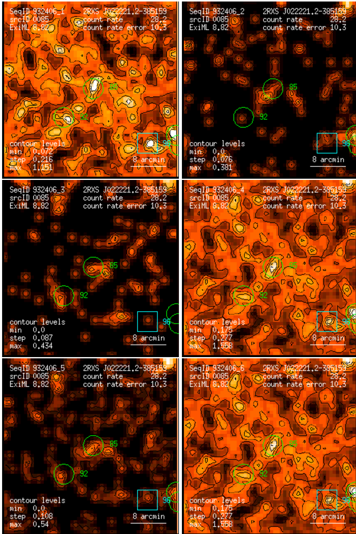
Figure 85: RASS 932406: detection 0085: band rate images, Gaussian filter: (1) PSPC channels 11 – 41, (2) 52 – 90, (3) 91 – 201, (4) 11 – 235, (5) 52 – 201, (6) 11 – 201. Broad band rates in counts/ks. Band rate contour levels in counts/ks/arcmin 2 .
