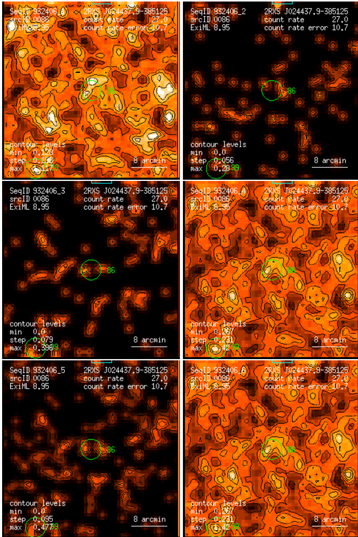
Figure 86: RASS 932406: detection 0086: band rate images, Gaussian filter: (1) PSPC channels 11 – 41, (2) 52 – 90, (3) 91 – 201, (4) 11 – 235, (5) 52 – 201, (6) 11 – 201. Broad band rates in counts/ks. Band rate contour levels in counts/ks/arcmin 2 .
