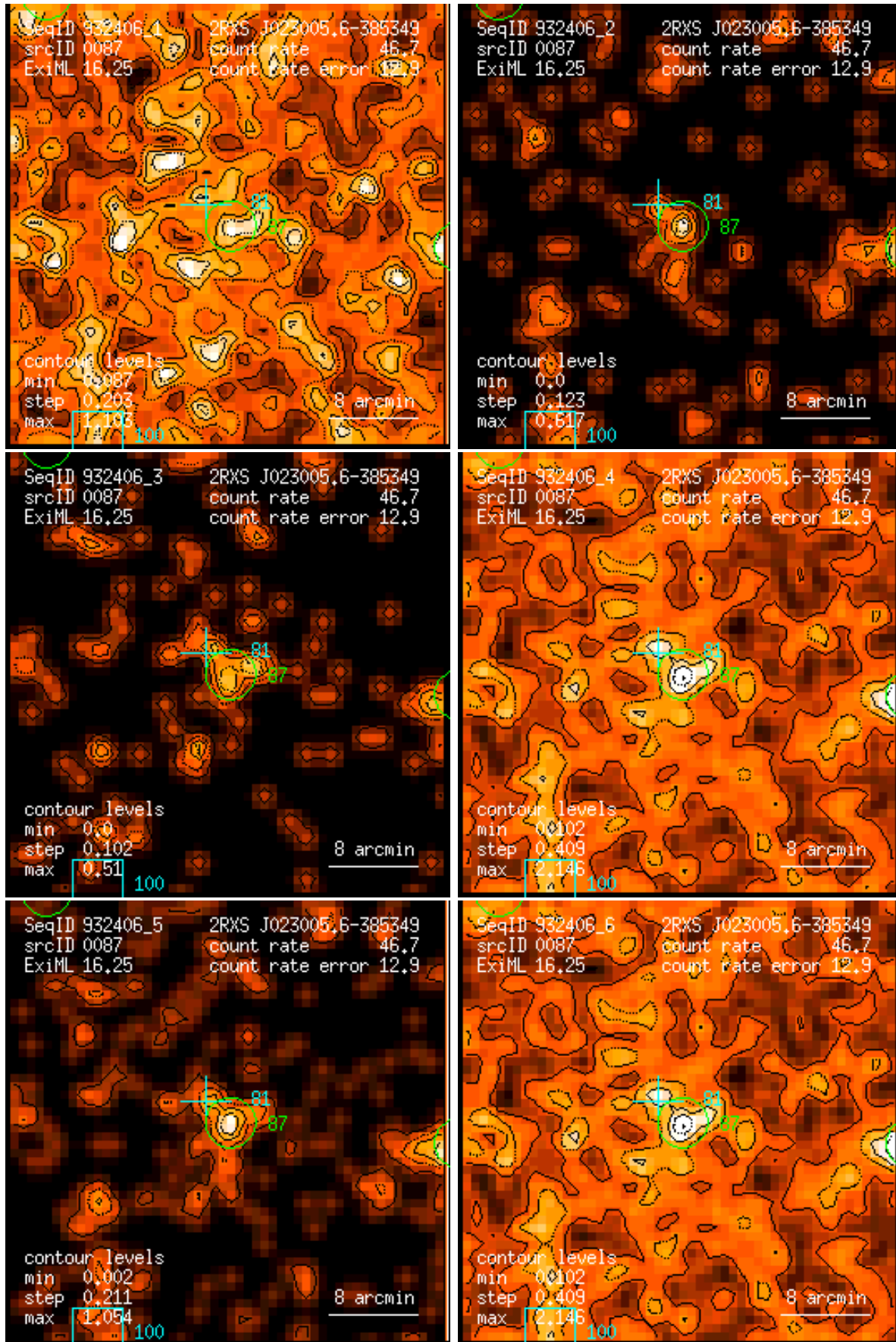
Figure 87: RASS 932406: detection 0087: band rate images, Gaussian filter: (1) PSPC channels 11 – 41, (2) 52 – 90, (3) 91 – 201, (4) 11 – 235, (5) 52 – 201, (6) 11 – 201. Broad band rates in counts/ks. Band rate contour levels in counts/ks/arcmin 2 .
