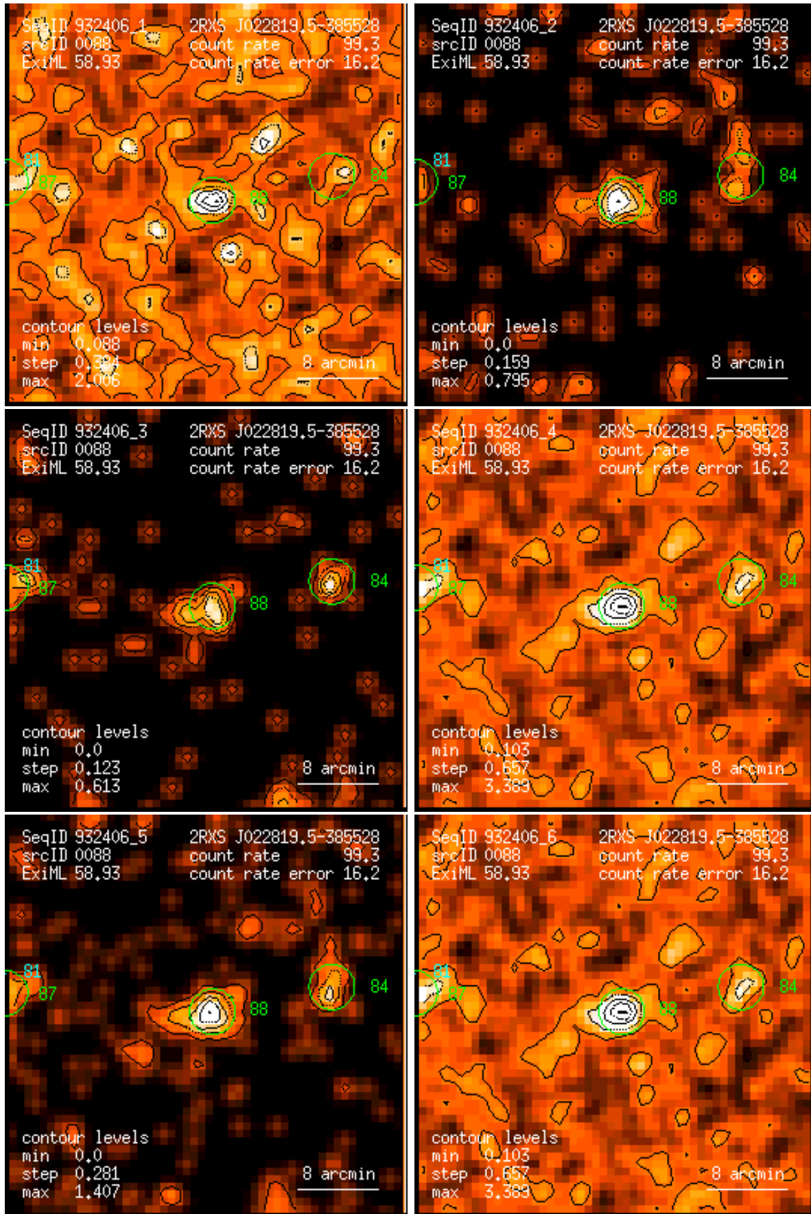
Figure 88: RASS 932406: detection 0088: band rate images, Gaussian filter: (1) PSPC channels 11 – 41, (2) 52 – 90, (3) 91 – 201, (4) 11 – 235, (5) 52 – 201, (6) 11 – 201. Broad band rates in counts/ks. Band rate contour levels in counts/ks/arcmin 2 .
