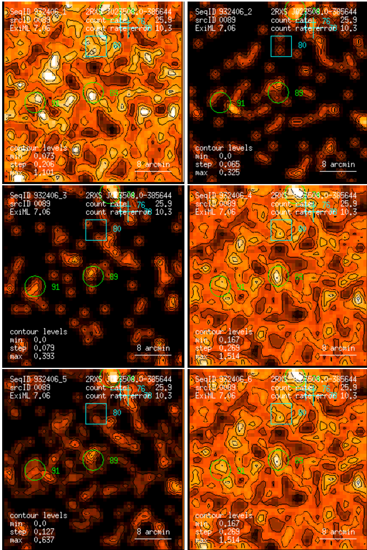
Figure 89: RASS 932406: detection 0089: band rate images, Gaussian filter: (1) PSPC channels 11 – 41, (2) 52 – 90, (3) 91 – 201, (4) 11 – 235, (5) 52 – 201, (6) 11 – 201. Broad band rates in counts/ks. Band rate contour levels in counts/ks/arcmin 2 .
