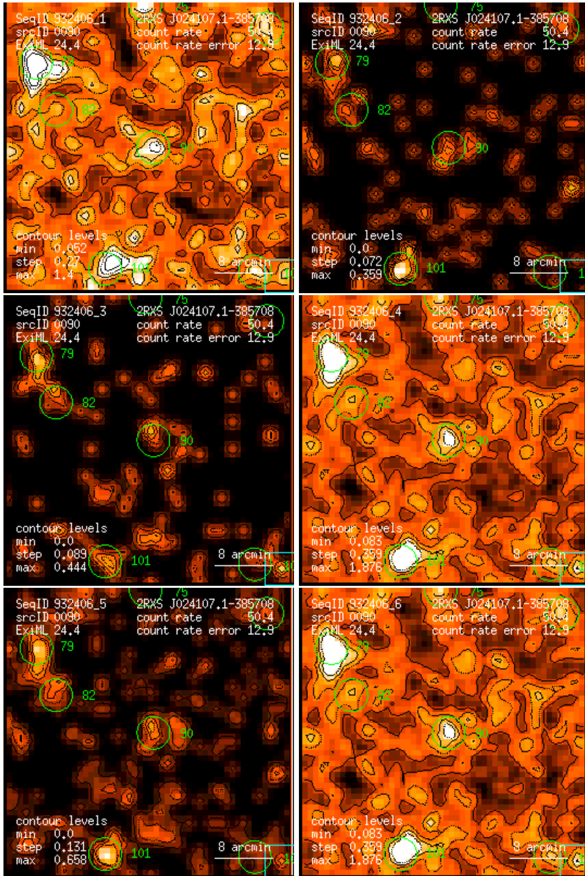
Figure 90: RASS 932406: detection 0090: band rate images, Gaussian filter: (1) PSPC channels 11 – 41, (2) 52 – 90, (3) 91 – 201, (4) 11 – 235, (5) 52 – 201, (6) 11 – 201. Broad band rates in counts/ks. Band rate contour levels in counts/ks/arcmin 2 .
