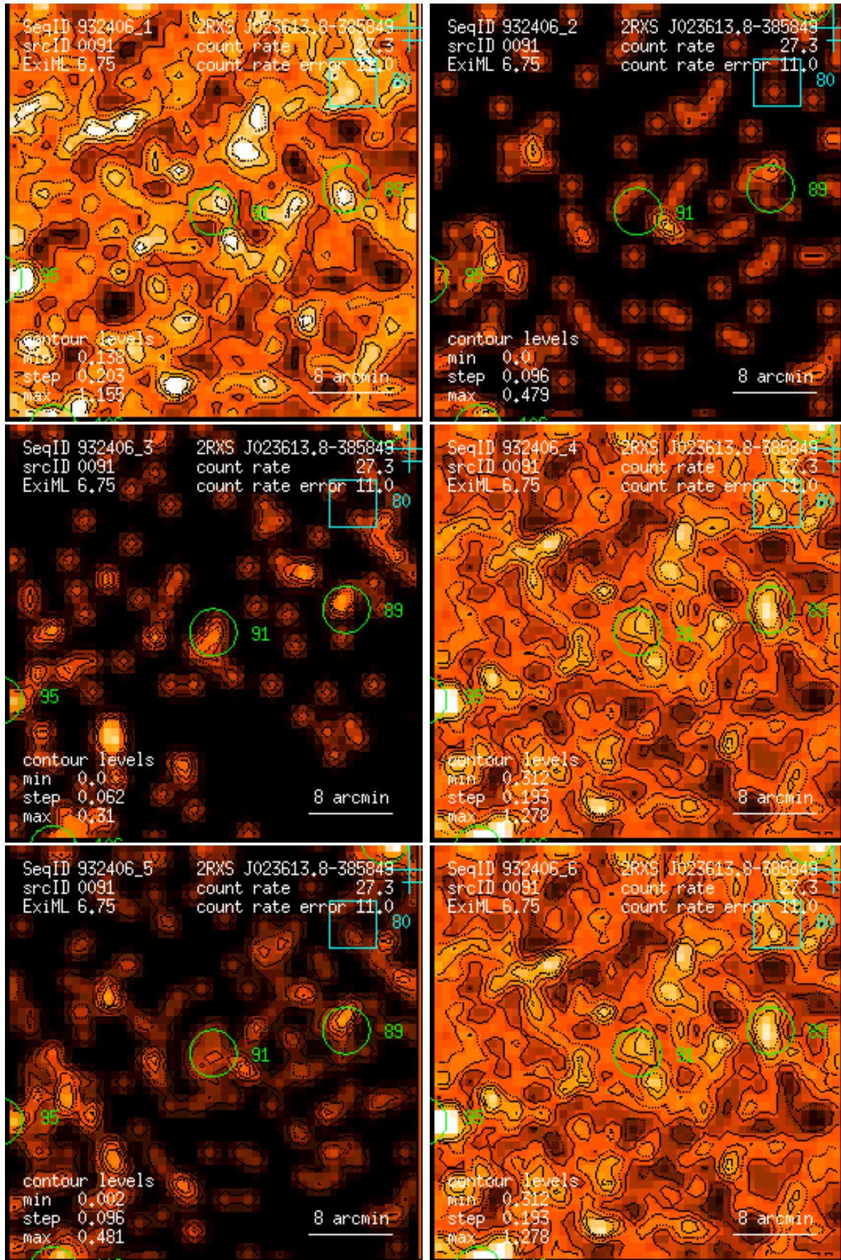
Figure 91: RASS 932406: detection 0091: band rate images, Gaussian filter: (1) PSPC channels 11 – 41, (2) 52 – 90, (3) 91 – 201, (4) 11 – 235, (5) 52 – 201, (6) 11 – 201. Broad band rates in counts/ks. Band rate contour levels in counts/ks/arcmin 2 .
