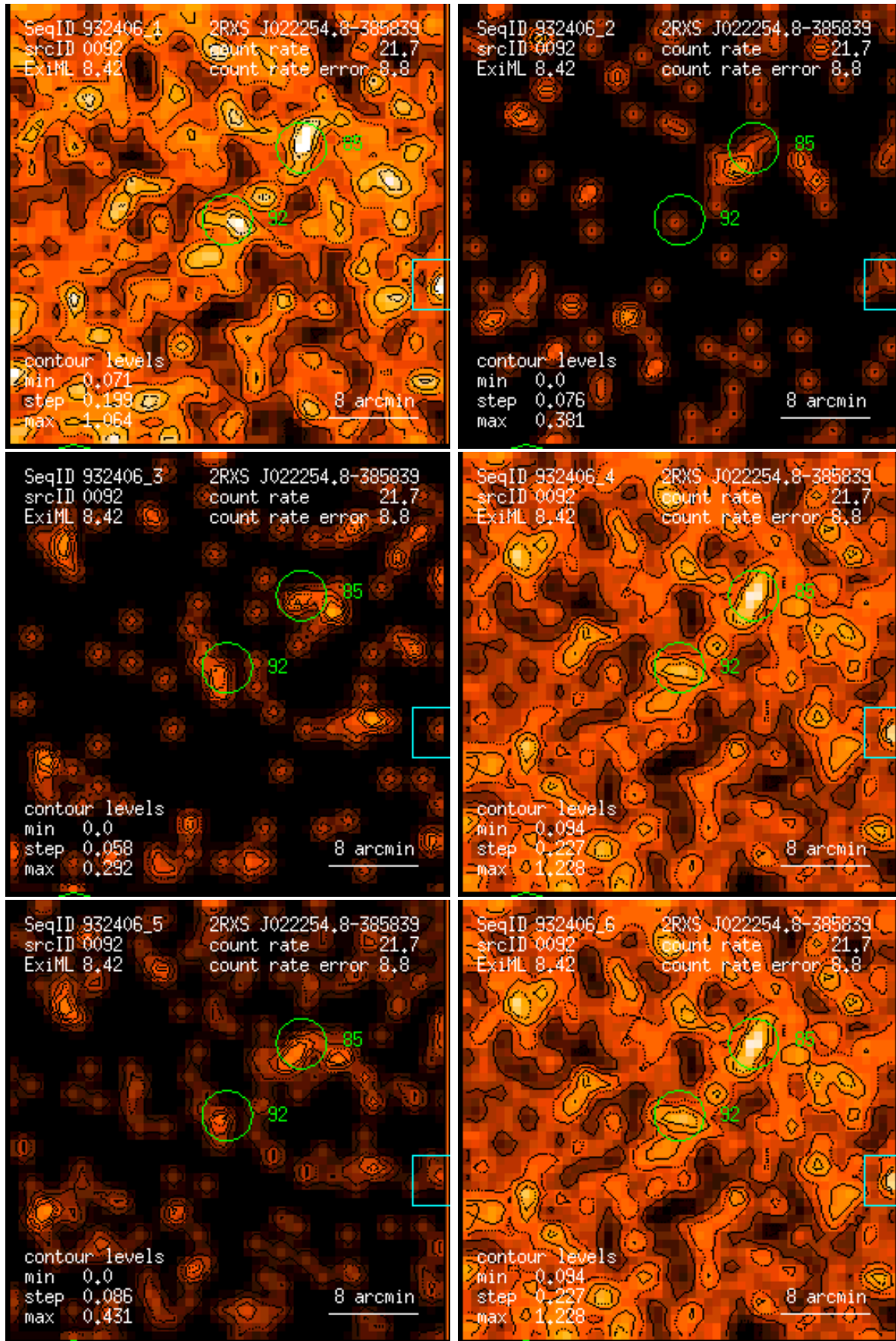
Figure 92: RASS 932406: detection 0092: band rate images, Gaussian filter: (1) PSPC channels 11 – 41, (2) 52 – 90, (3) 91 – 201, (4) 11 – 235, (5) 52 – 201, (6) 11 – 201. Broad band rates in counts/ks. Band rate contour levels in counts/ks/arcmin 2 .
