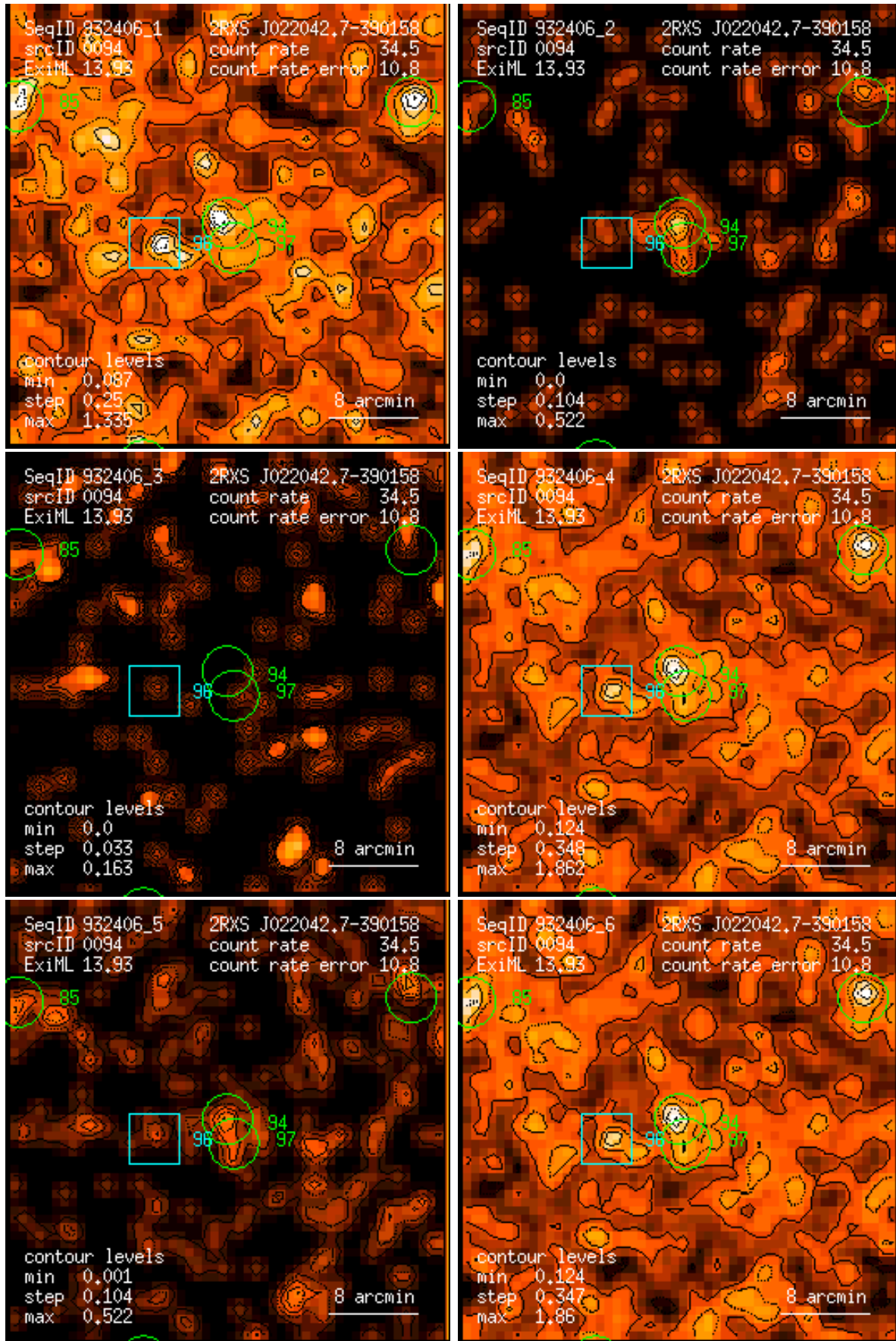
Figure 94: RASS 932406: detection 0094: band rate images, Gaussian filter: (1) PSPC channels 11 – 41, (2) 52 – 90, (3) 91 – 201, (4) 11 – 235, (5) 52 – 201, (6) 11 – 201. Broad band rates in counts/ks. Band rate contour levels in counts/ks/arcmin 2 .
