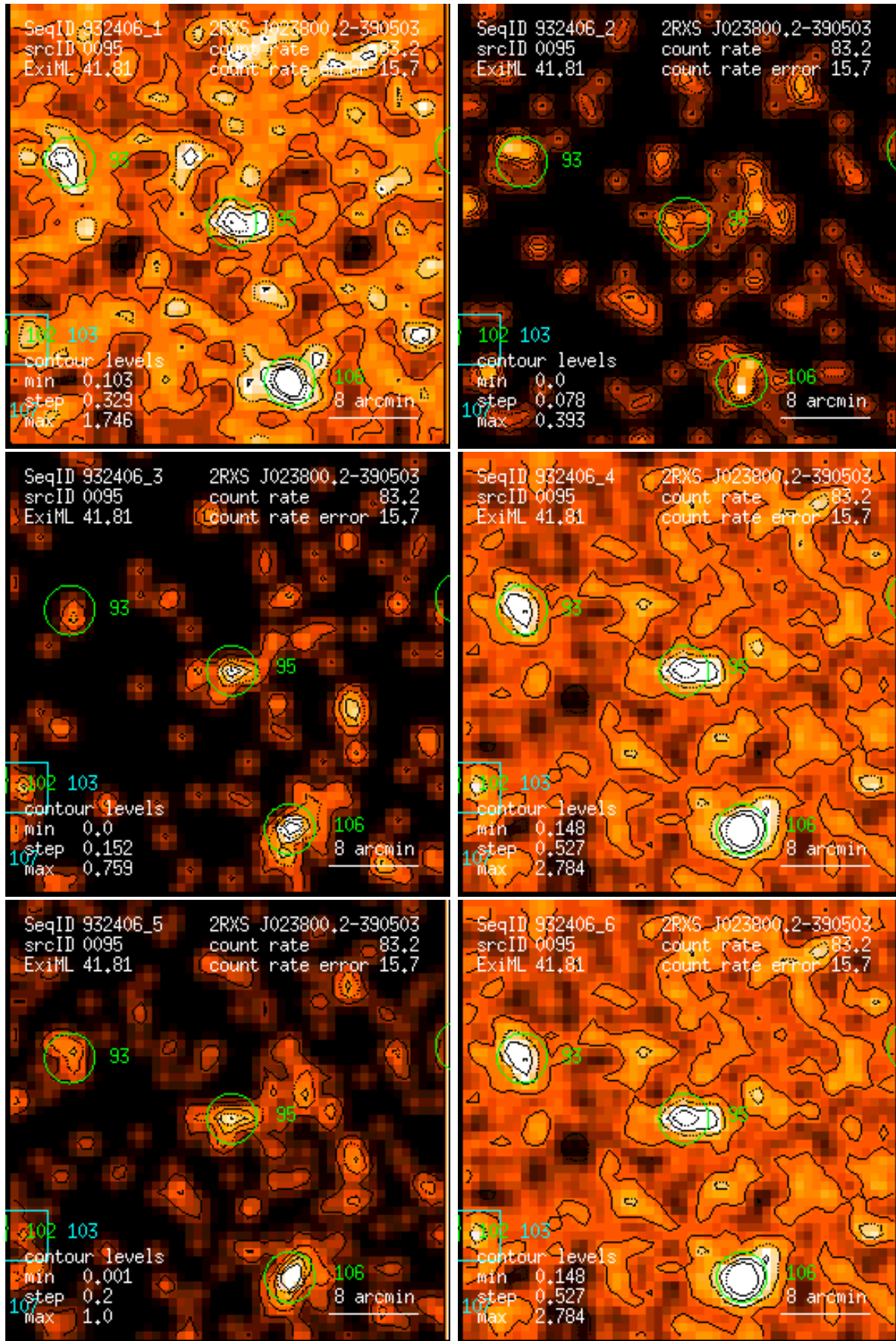
Figure 95: RASS 932406: detection 0095: band rate images, Gaussian filter: (1) PSPC channels 11 – 41, (2) 52 – 90, (3) 91 – 201, (4) 11 – 235, (5) 52 – 201, (6) 11 – 201. Broad band rates in counts/ks. Band rate contour levels in counts/ks/arcmin 2 .
