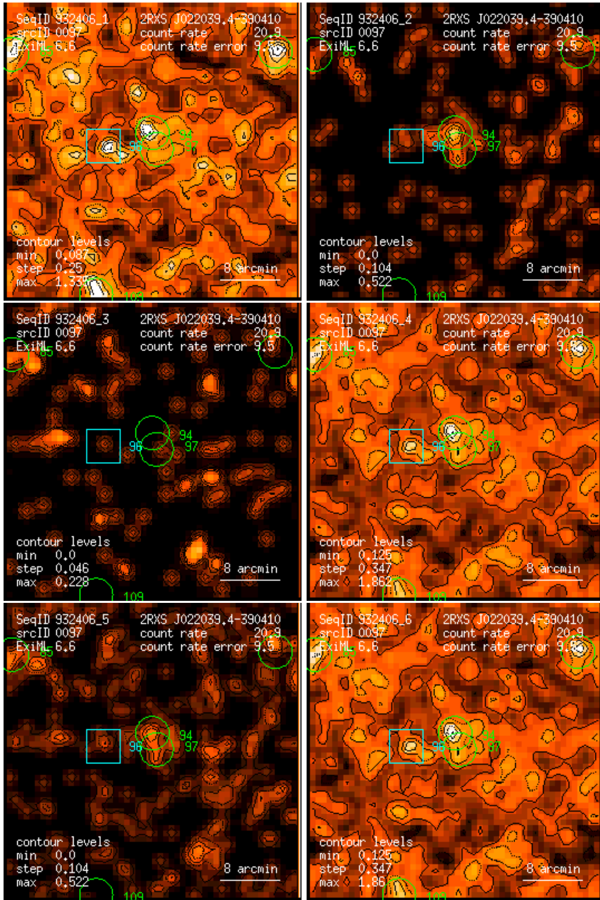
Figure 97: RASS 932406: detection 0097: band rate images, Gaussian filter: (1) PSPC channels 11 – 41, (2) 52 – 90, (3) 91 – 201, (4) 11 – 235, (5) 52 – 201, (6) 11 – 201. Broad band rates in counts/ks. Band rate contour levels in counts/ks/arcmin 2 .
