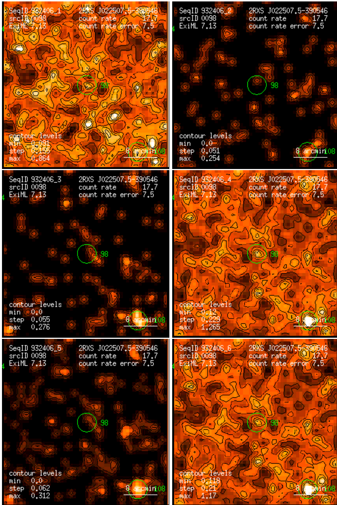
Figure 98: RASS 932406: detection 0098: band rate images, Gaussian filter: (1) PSPC channels 11 – 41, (2) 52 – 90, (3) 91 – 201, (4) 11 – 235, (5) 52 – 201, (6) 11 – 201. Broad band rates in counts/ks. Band rate contour levels in counts/ks/arcmin 2 .
