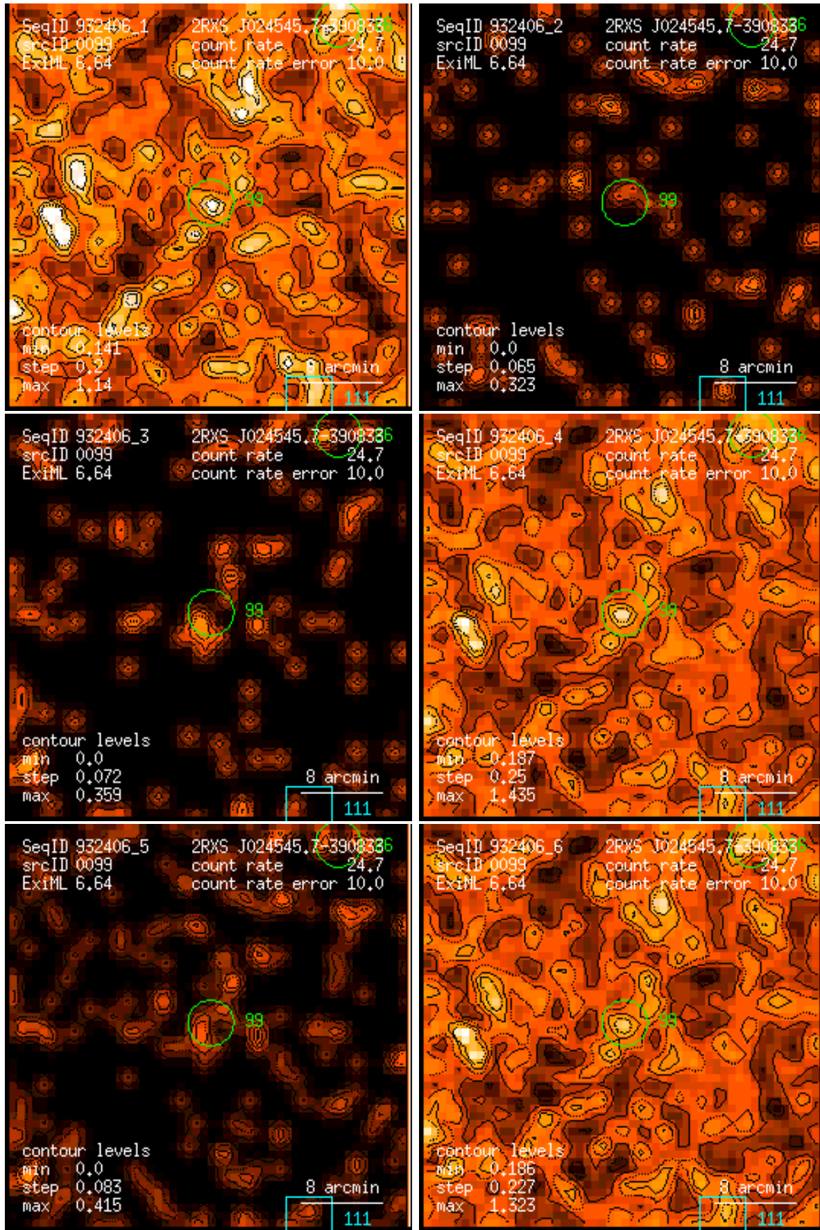
Figure 99: RASS 932406: detection 0099: band rate images, Gaussian filter: (1) PSPC channels 11 – 41, (2) 52 – 90, (3) 91 – 201, (4) 11 – 235, (5) 52 – 201, (6) 11 – 201. Broad band rates in counts/ks. Band rate contour levels in counts/ks/arcmin 2 .
