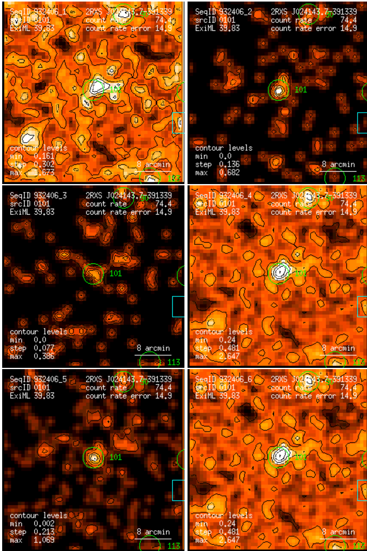
Figure 101: RASS 932406: detection 0101: band rate images, Gaussian filter: (1) PSPC channels 11 – 41, (2) 52 – 90, (3) 91 – 201, (4) 11 – 235, (5) 52 – 201, (6) 11 – 201. Broad band rates in counts/ks. Band rate contour levels in counts/ks/arcmin 2 .
