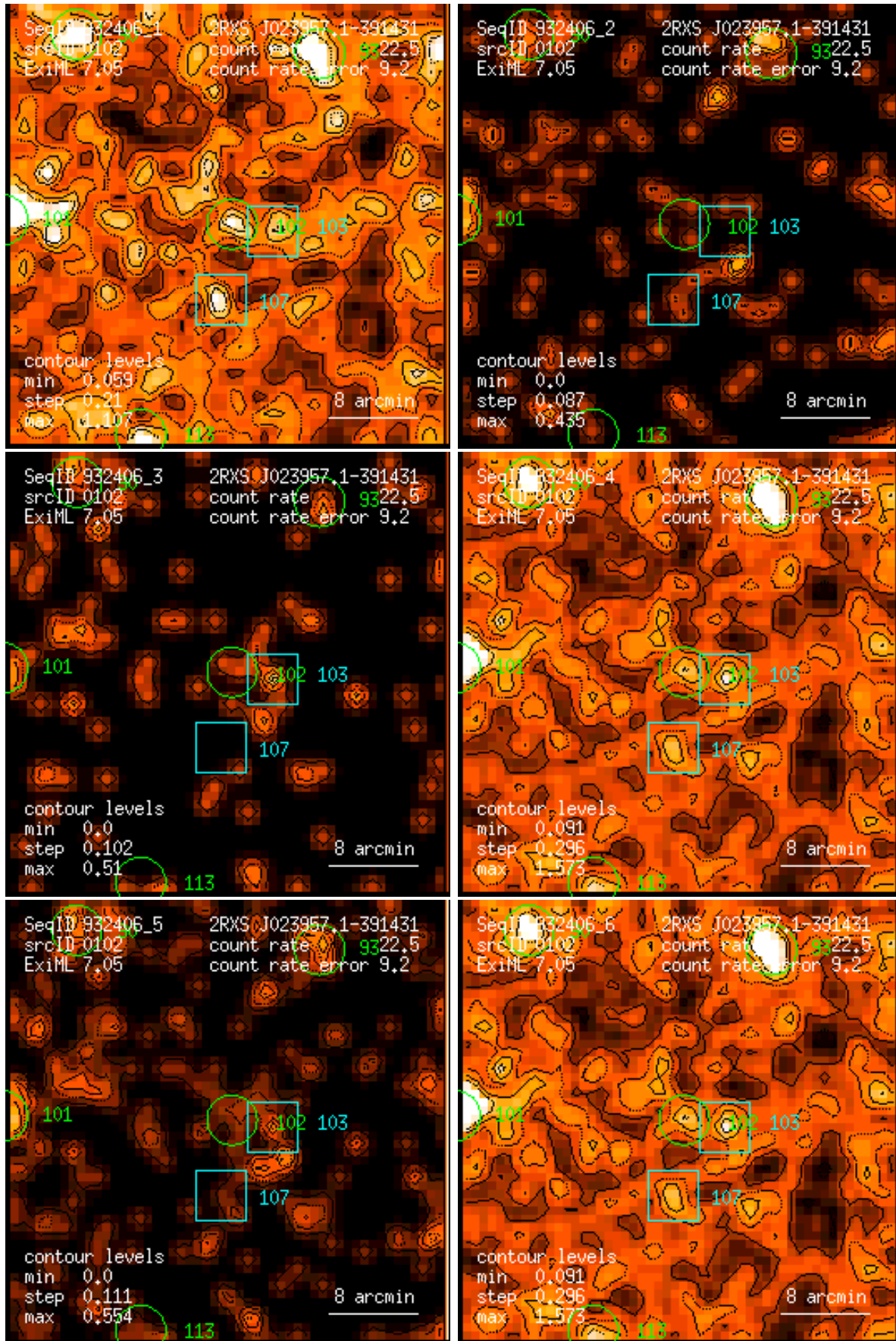
Figure 102: RASS 932406: detection 0102: band rate images, Gaussian filter: (1) PSPC channels 11 – 41, (2) 52 – 90, (3) 91 – 201, (4) 11 – 235, (5) 52 – 201, (6) 11 – 201. Broad band rates in counts/ks. Band rate contour levels in counts/ks/arcmin 2 .
