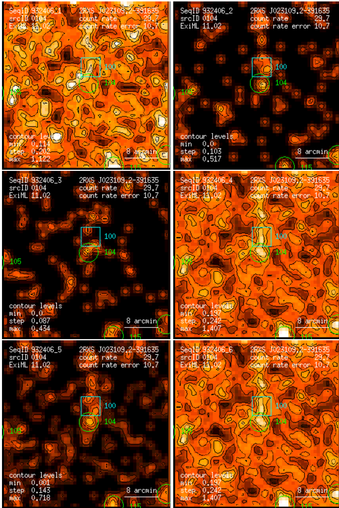
Figure 104: RASS 932406: detection 0104: band rate images, Gaussian filter: (1) PSPC channels 11 – 41, (2) 52 – 90, (3) 91 – 201, (4) 11 – 235, (5) 52 – 201, (6) 11 – 201. Broad band rates in counts/ks. Band rate contour levels in counts/ks/arcmin 2 .
