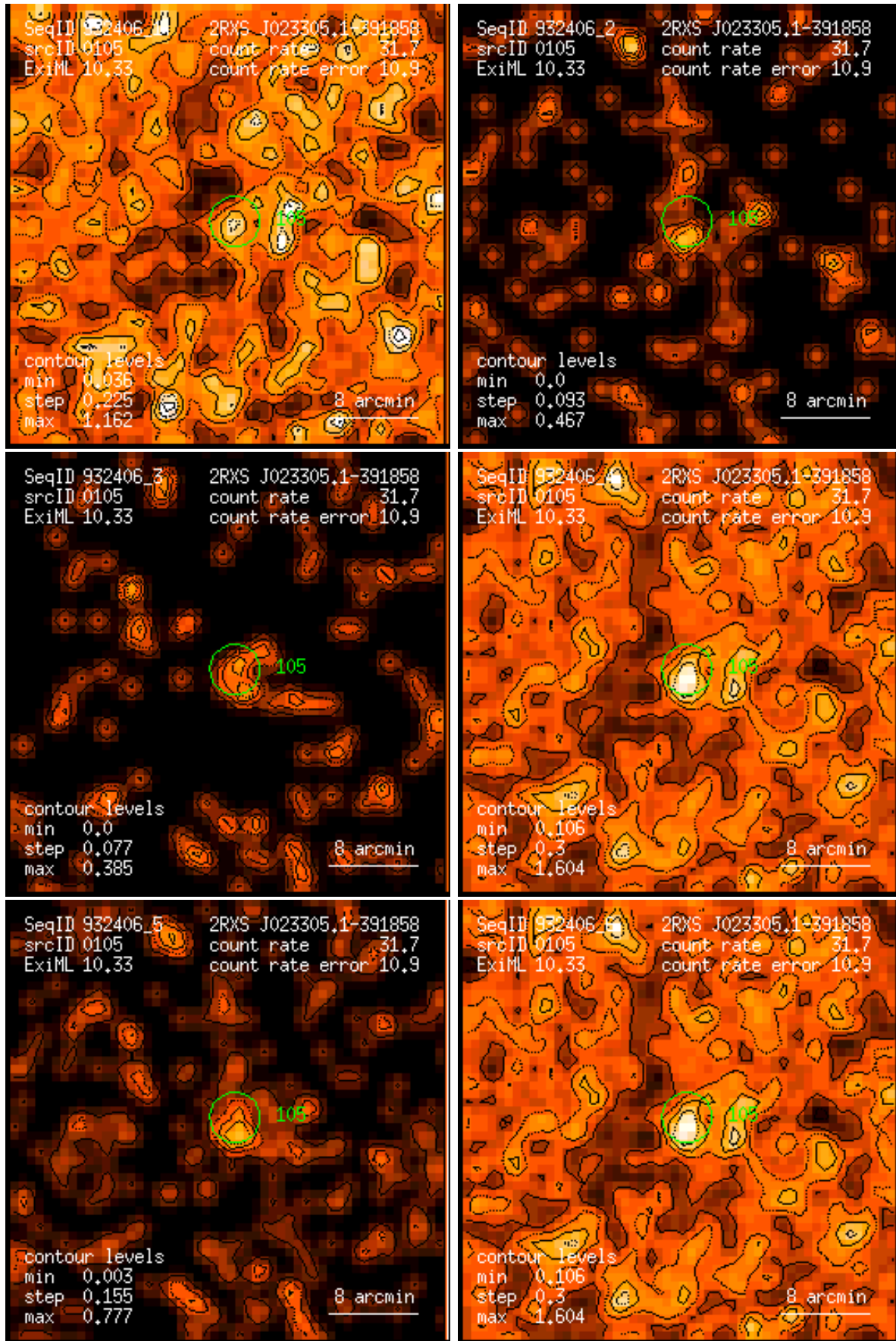
Figure 105: RASS 932406: detection 0105: band rate images, Gaussian filter: (1) PSPP channels 11 – 41, (2) 52 – 90, (3) 91 – 201, (4) 11 – 235, (5) 52 – 201, (6) 11 – 201. Broad band rates in counts/ks. Band rate contour levels in counts/ks/arcmin 2 .
