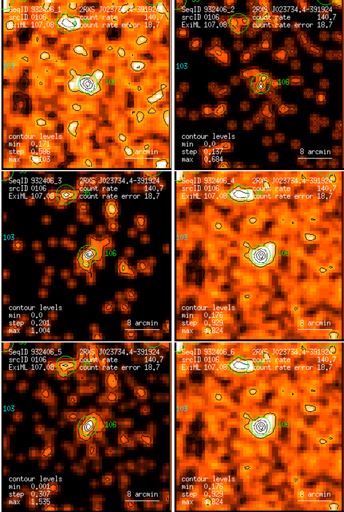
Figure 106: RASS 932406: detection 0106: band rate images, Gaussian filter: (1) PSPC channels 11 – 41, (2) 52 – 90, (3) 91 – 201, (4) 11 – 235, (5) 52 – 201, (6) 11 – 201. Broad band rates in counts/ks. Band rate contour levels in counts/ks/arcmin 2 .
