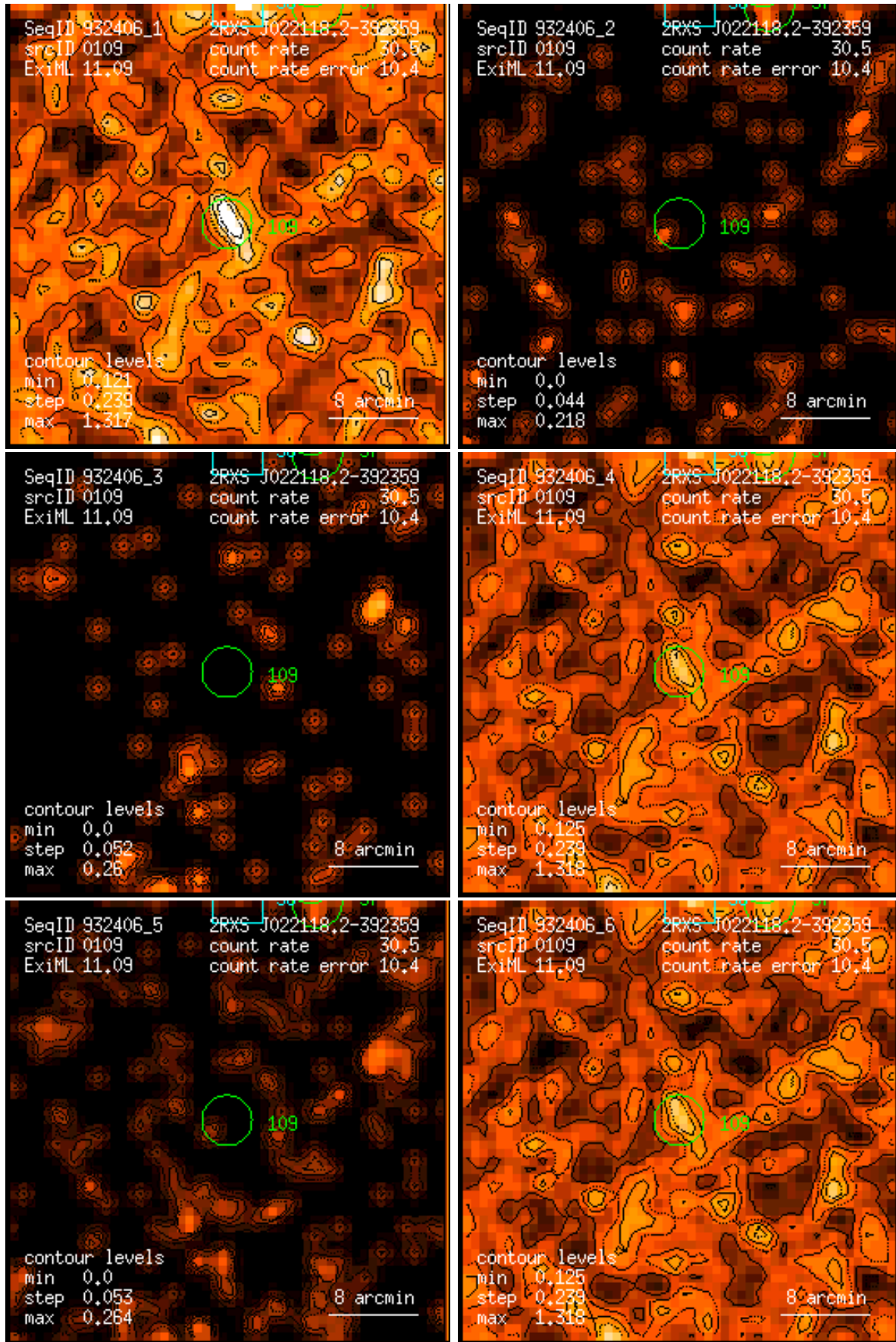
Figure 109: RASS 932406: detection 0109: band rate images, Gaussian filter: (1) PSPC channels 11 – 41, (2) 52 – 90, (3) 91 – 201, (4) 11 – 235, (5) 52 – 201, (6) 11 – 201. Broad band rates in counts/ks. Band rate contour levels in counts/ks/arcmin 2 .
