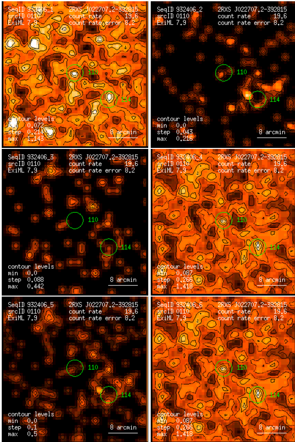
Figure 110: RASS 932406: detection 0110: band rate images, Gaussian filter: (1) PSPC channels 11 – 41, (2) 52 – 90, (3) 91 – 201, (4) 11 – 235, (5) 52 – 201, (6) 11 – 201. Broad band rates in counts/ks. Band rate contour levels in counts/ks/arcmin 2 .
