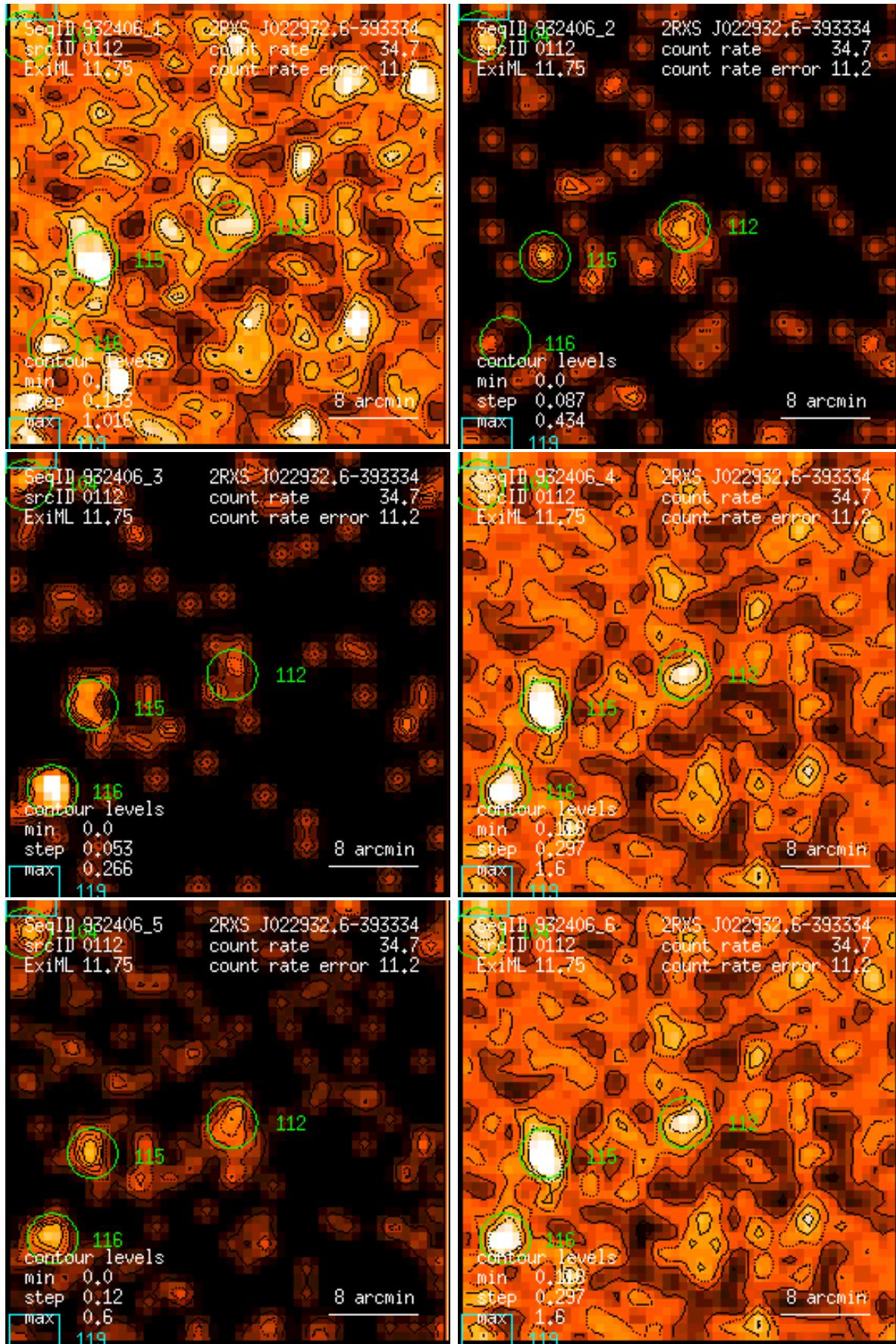
Figure 112: RASS 932406: detection 0112: band rate images, Gaussian filter: (1) PSPC channels 11 – 41, (2) 52 – 90, (3) 91 – 201, (4) 11 – 235, (5) 52 – 201, (6) 11 – 201. Broad band rates in counts/ks. Band rate contour levels in counts/ks/arcmin 2 .
