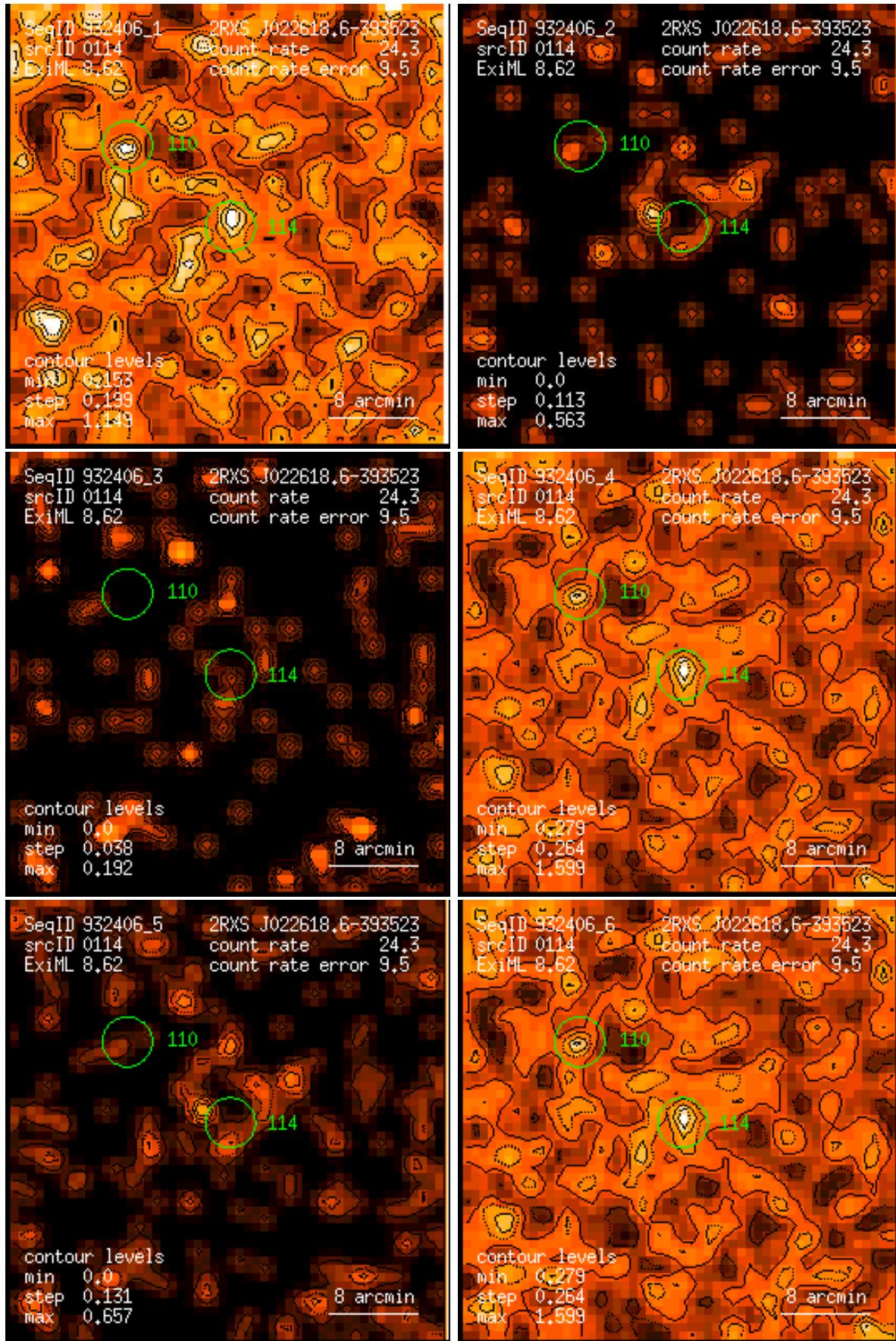
Figure 114: RASS 932406: detection 0114: band rate images, Gaussian filter: (1) PSPC channels 11 – 41, (2) 52 – 90, (3) 91 – 201, (4) 11 – 235, (5) 52 – 201, (6) 11 – 201. Broad band rates in counts/ks. Band rate contour levels in counts/ks/arcmin 2 .
