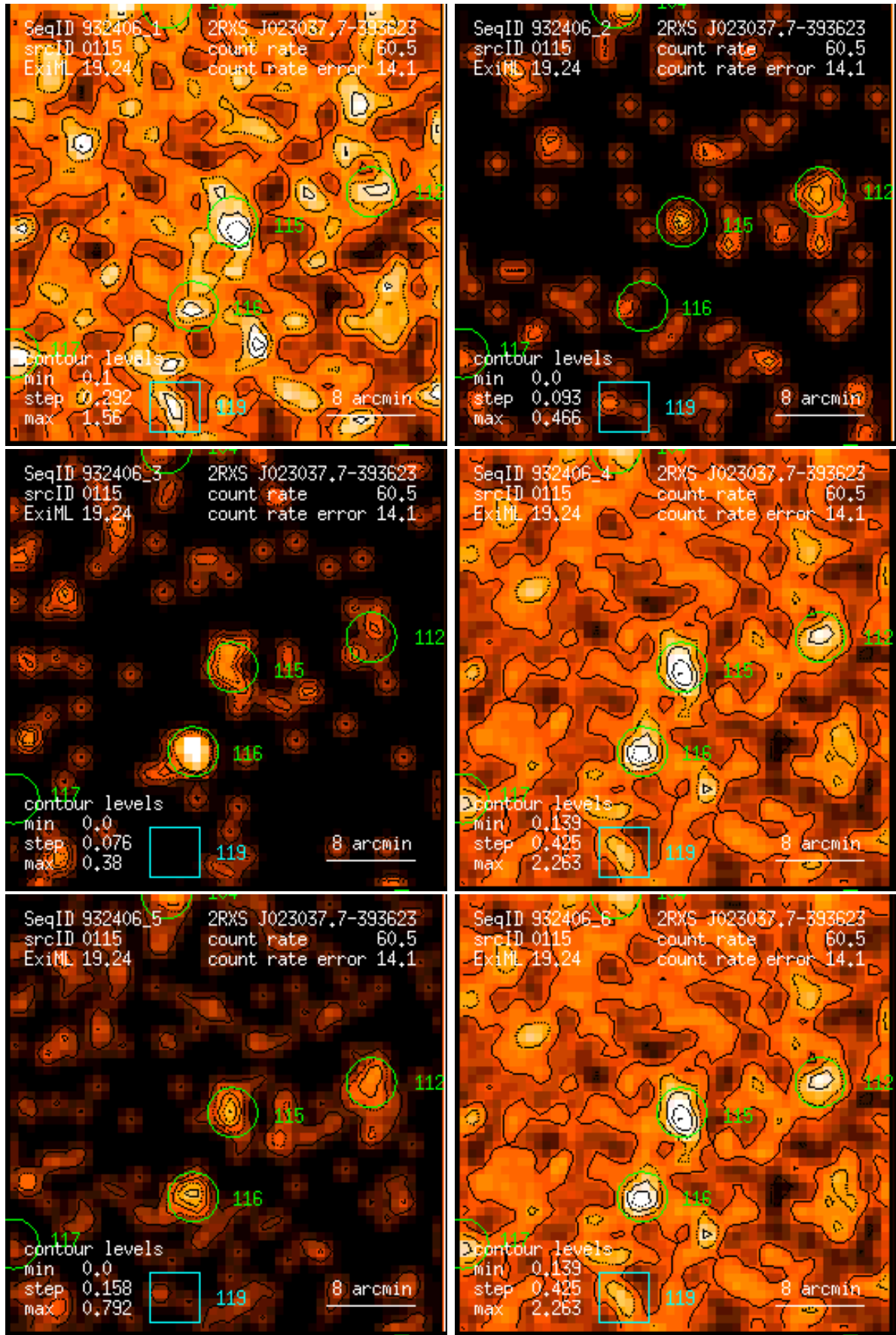
Figure 115: RASS 932406: detection 0115: band rate images, Gaussian filter: (1) PSPC channels 11 – 41, (2) 52 – 90, (3) 91 – 201, (4) 11 – 235, (5) 52 – 201, (6) 11 – 201. Broad band rates in counts/ks. Band rate contour levels in counts/ks/arcmin 2 .
